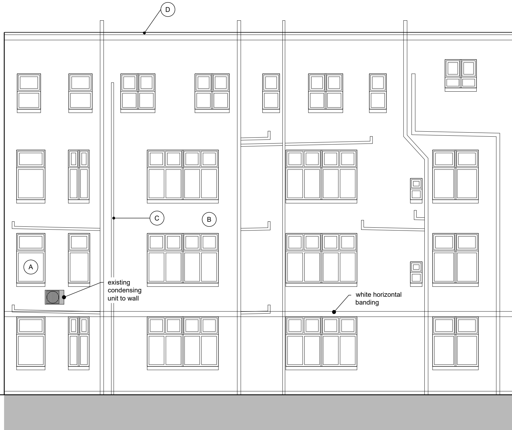
1 Existing - South-East Elevation
