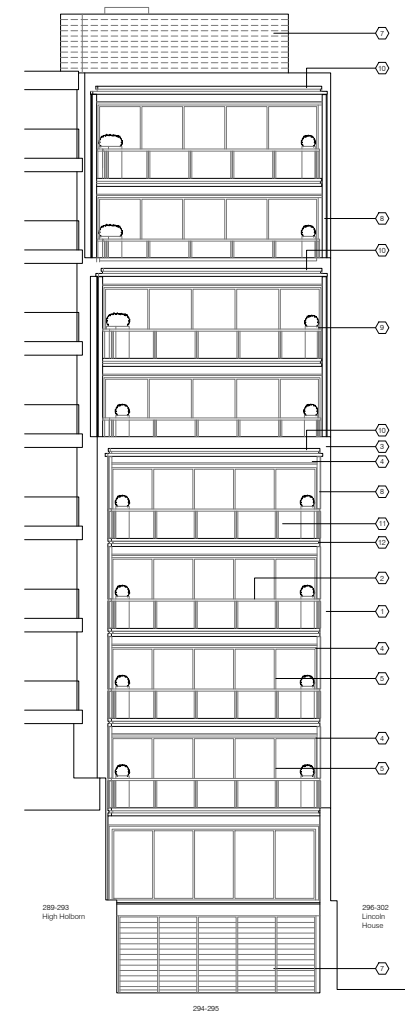
Proposed South Elevation - Elevation 5
