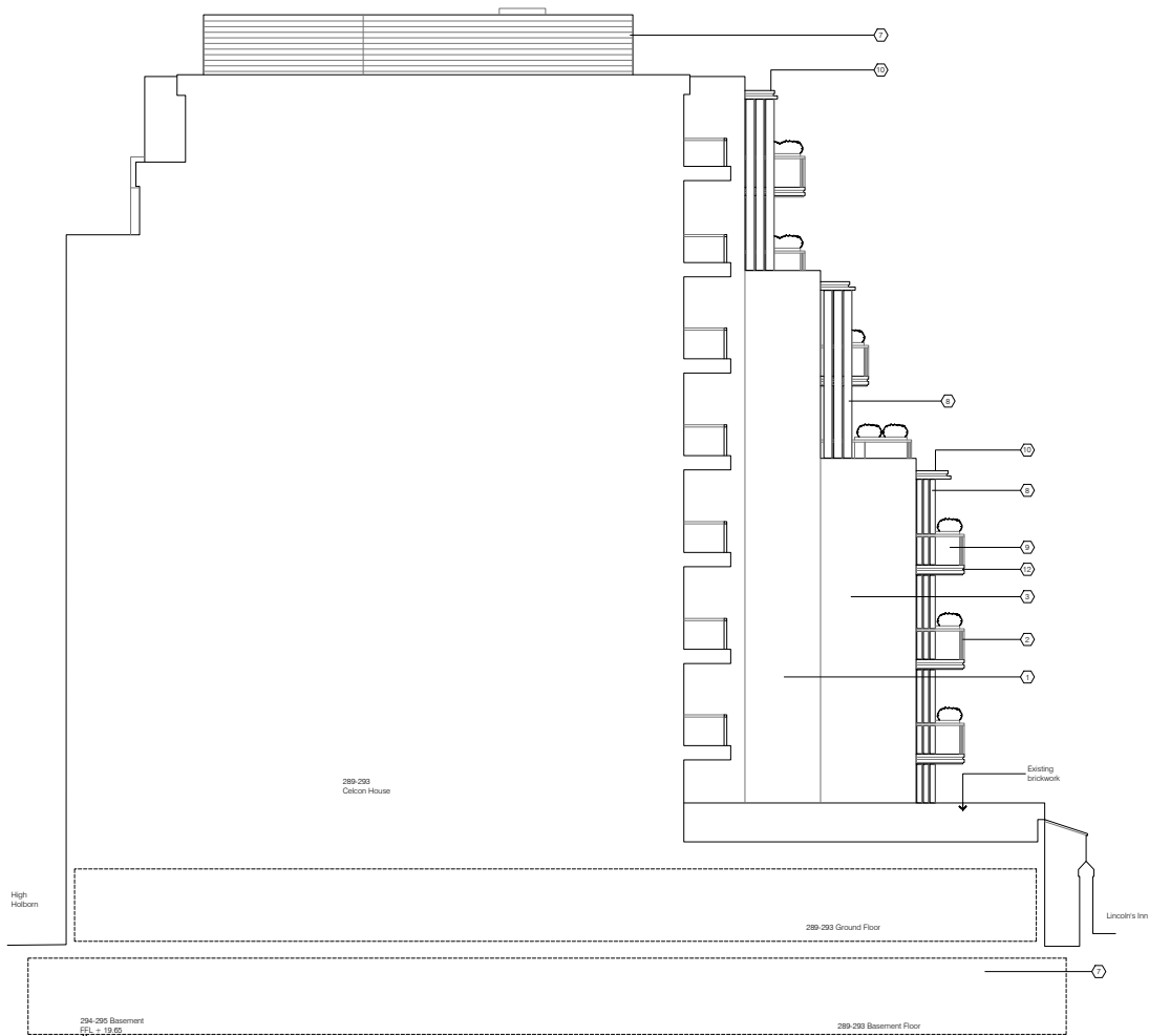
Proposed West Elevation - Elevation 3
