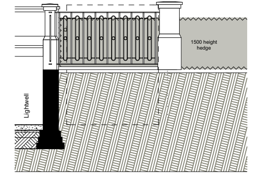
Elevation 1:100@A3
