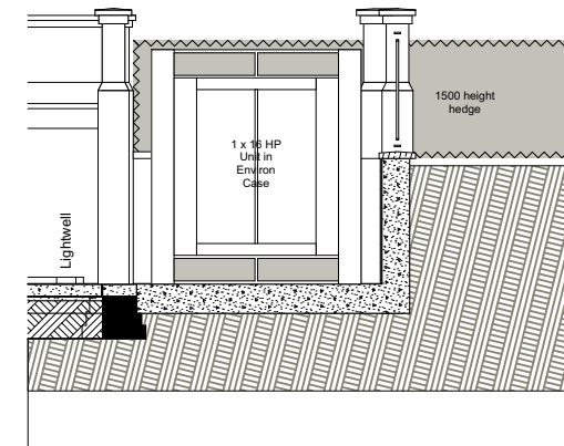
Section 1:100@A3
