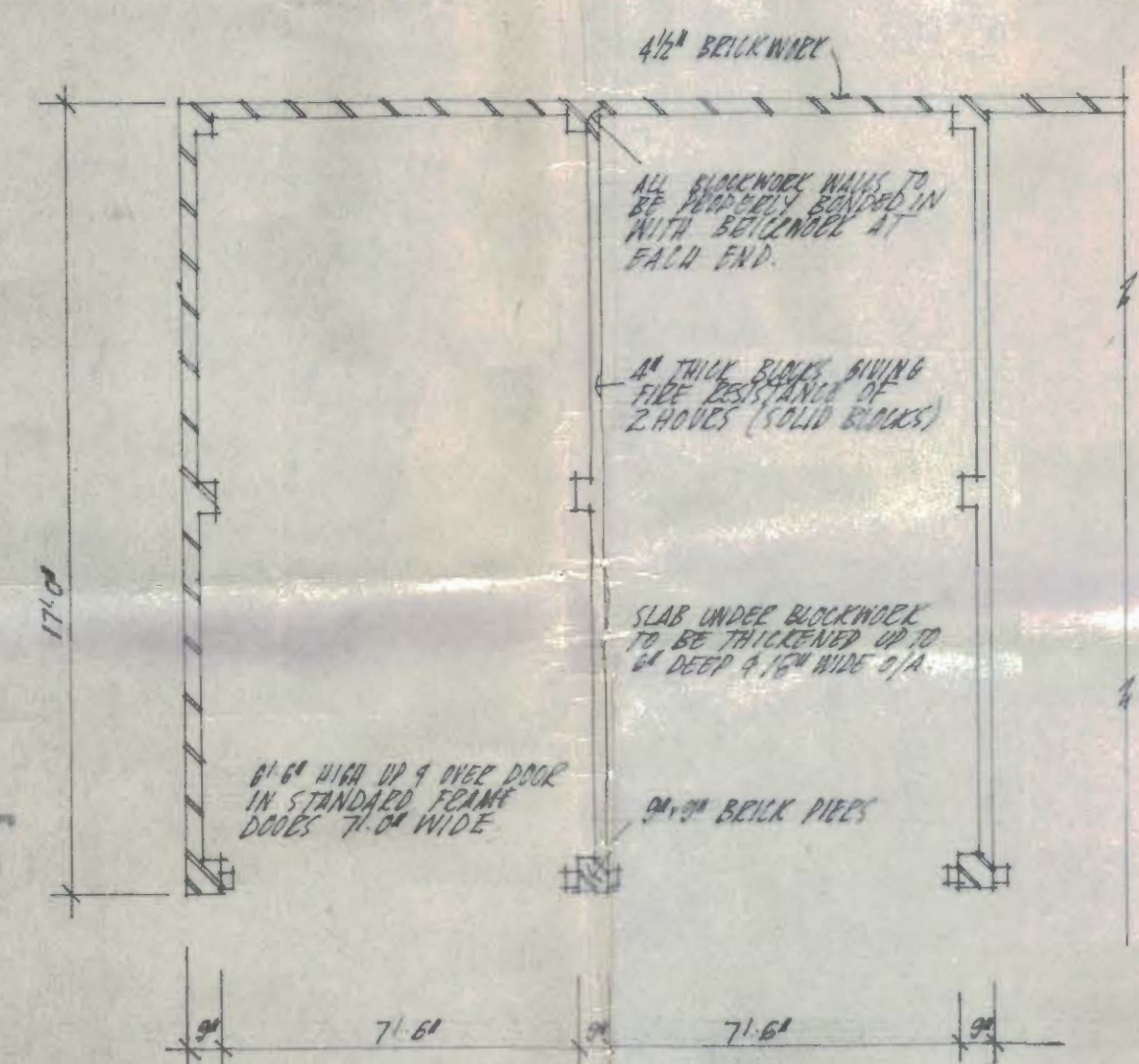
PLAN COMPOUND
