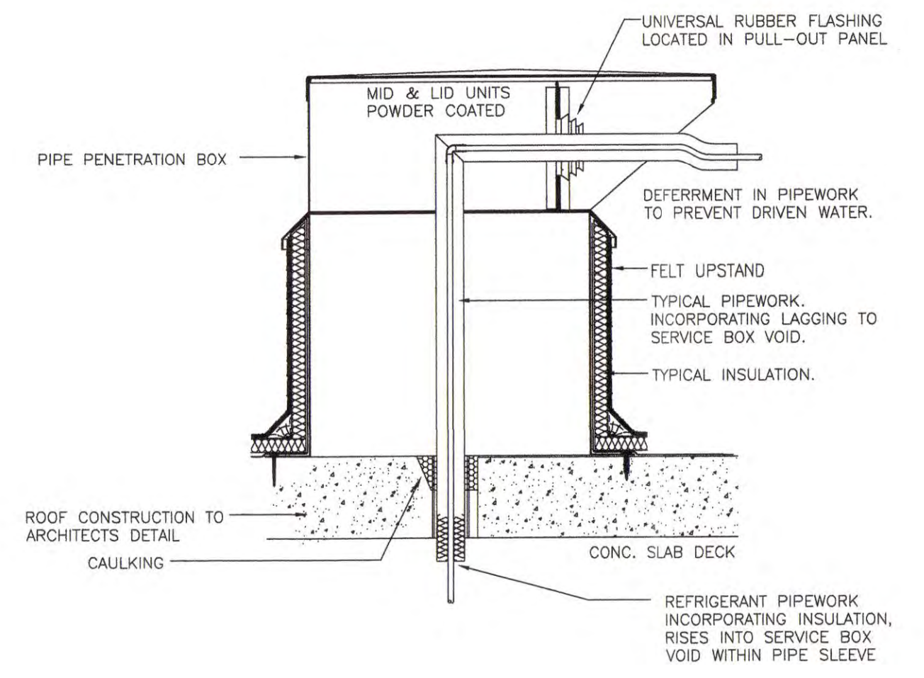
TYPICAL REFRIGERANT PIPEWORK ROOF PENETRATION DETAIL (SCALE 1:10)
