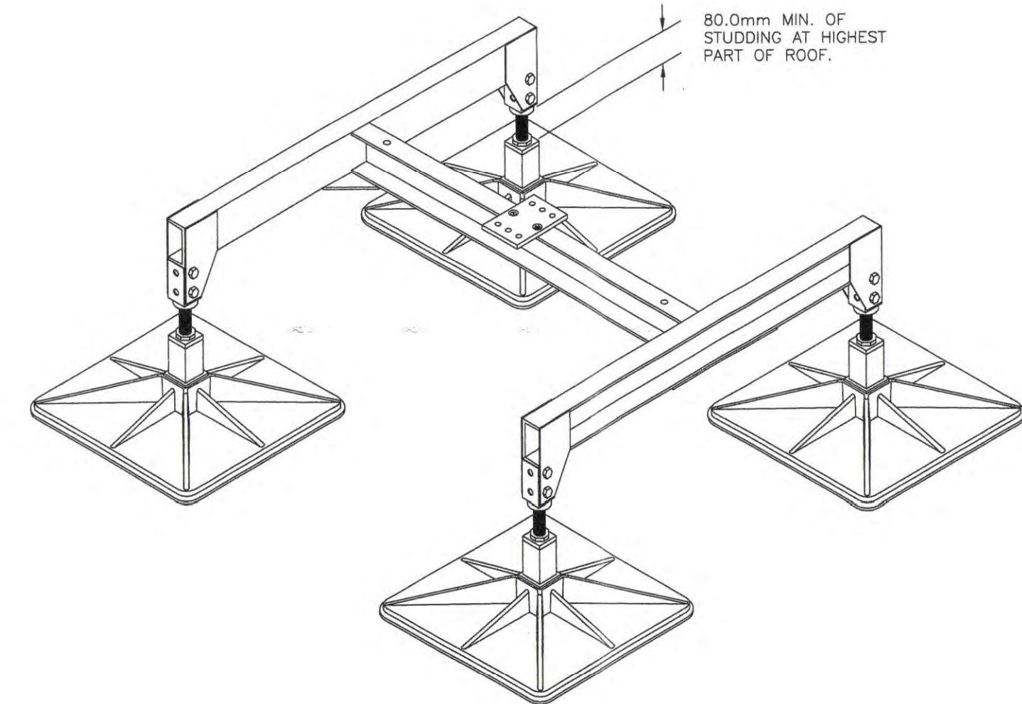
TYPICAL OUTDOOR UNIT SUPPORT DETAIL (SCALE 1:10)
