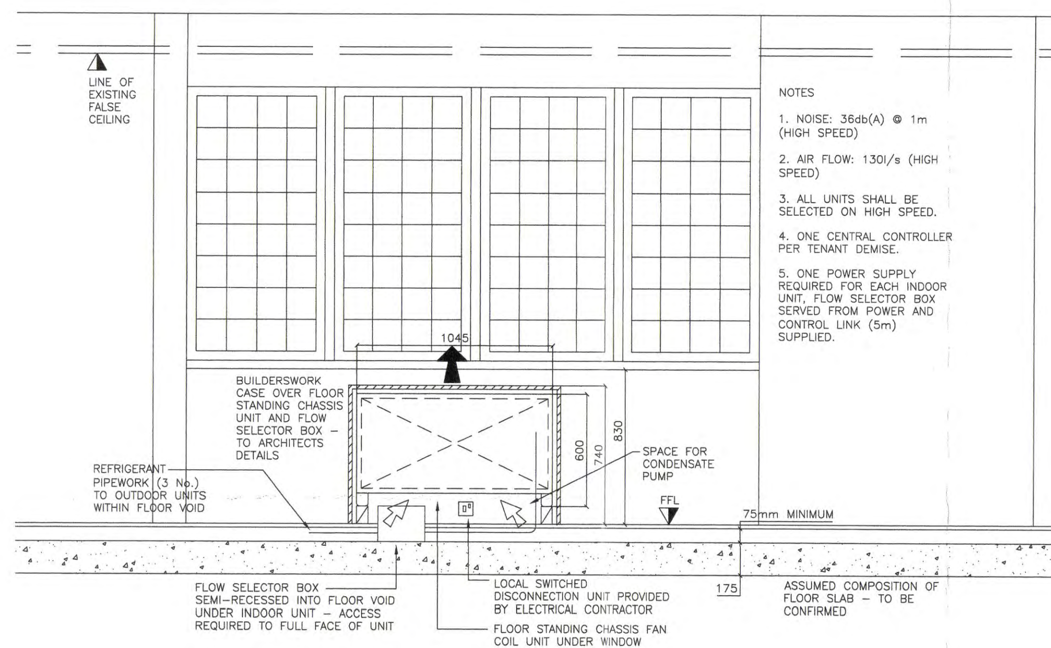
SECTION E-E TYPICAL FIRST FLOOR INTERNAL UNIT INSTALLATION (Scale 1:20)
