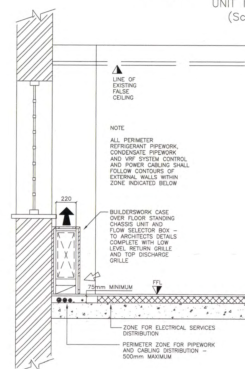
SECTION F-F TYPICAL SECTION THROUGH PERIMETER (Scale 1:20)
