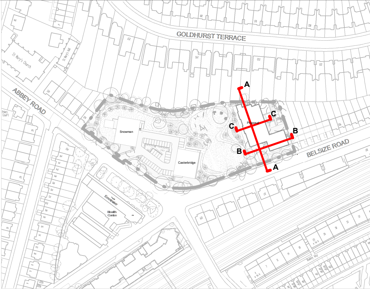
Key Plan 1:2000
