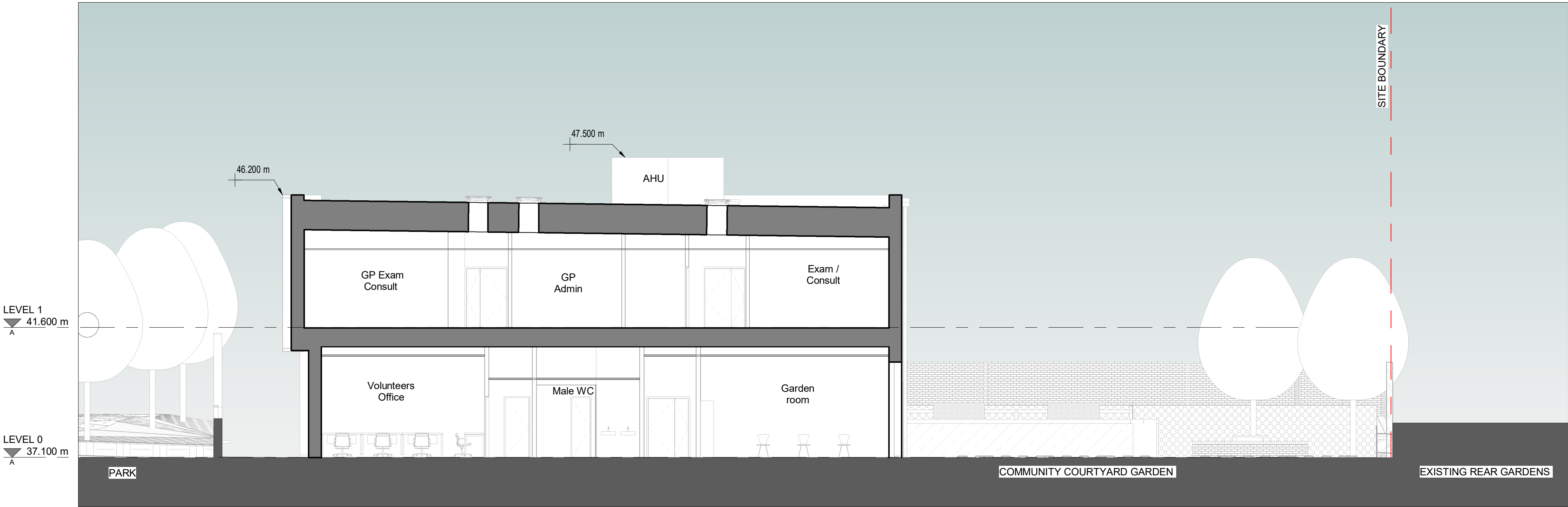
Section CC
