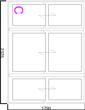
Double Glazed Timber Sash
