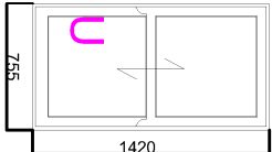
Double Glazed Timber Sash
