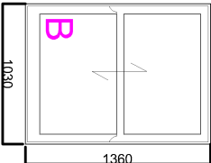
Double Glazed Timber Sash
