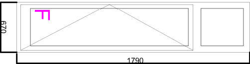
Double Glazed Timber Sash
