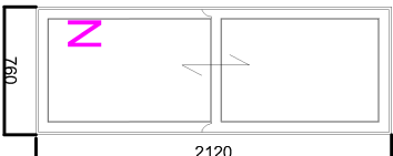
Double Glazed Timber Sash
