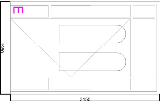
Double Glazed Timber Door
