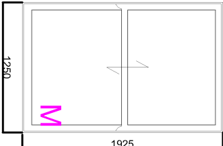
Double Glazed Timber Sash
