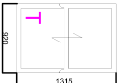
Single Glazed Timber Sash
