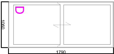
Single Glazed Timber Sash
