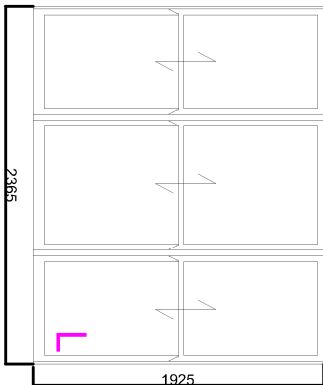
Single Glazed Timber Sash
