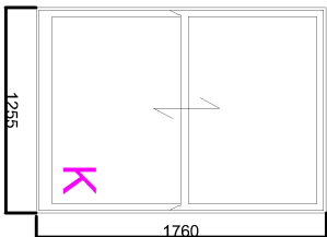
Single Glazed Timber Sash
