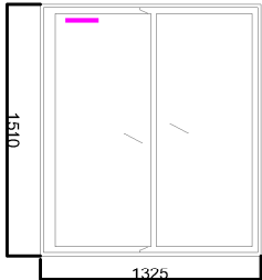
Single Glazed Timber Sash
