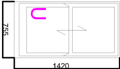
Single Glazed Timber Sash
