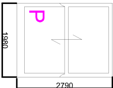
Single Glazed Timber Sash
