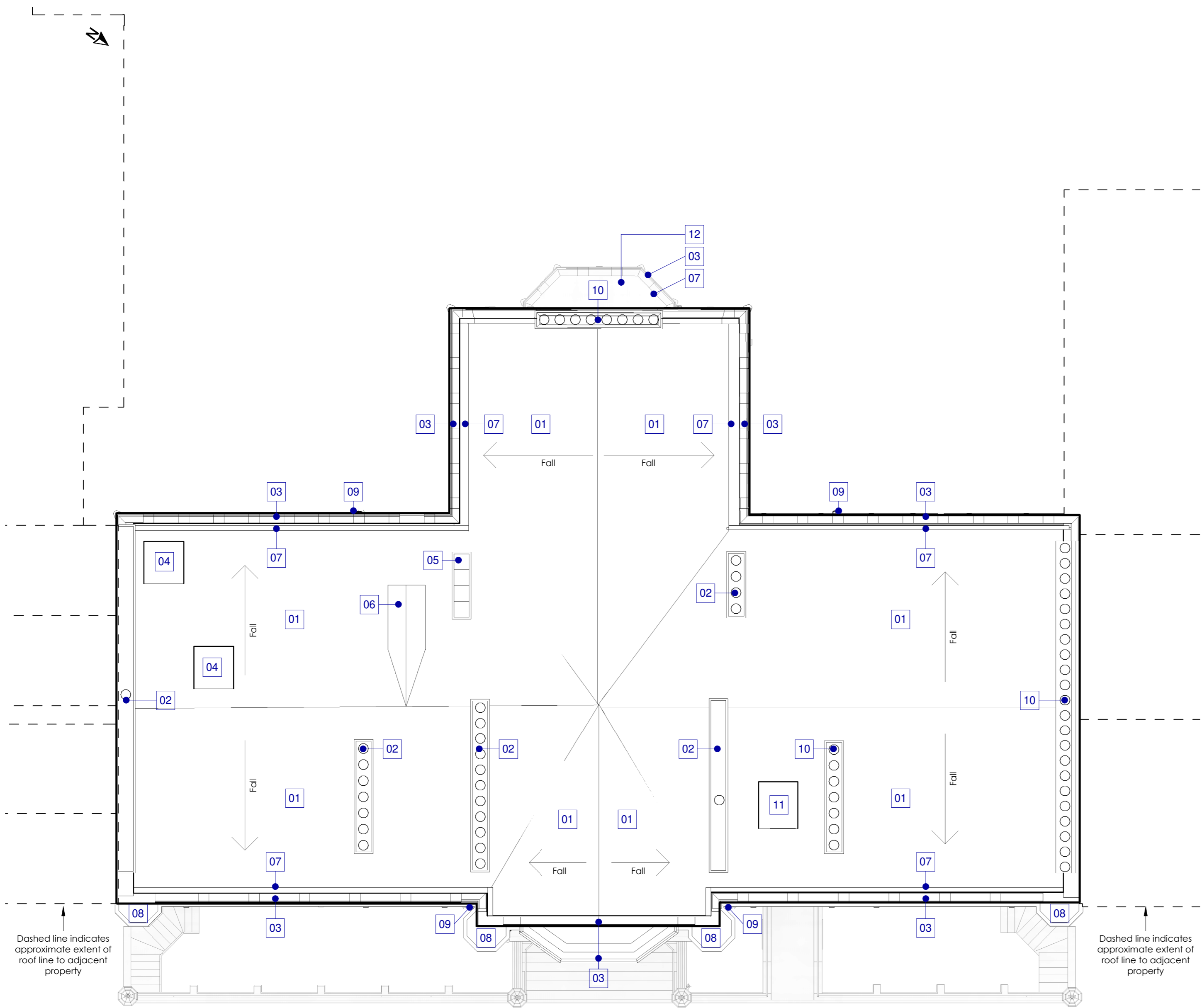
Existing Roof Plan 1 : 100
