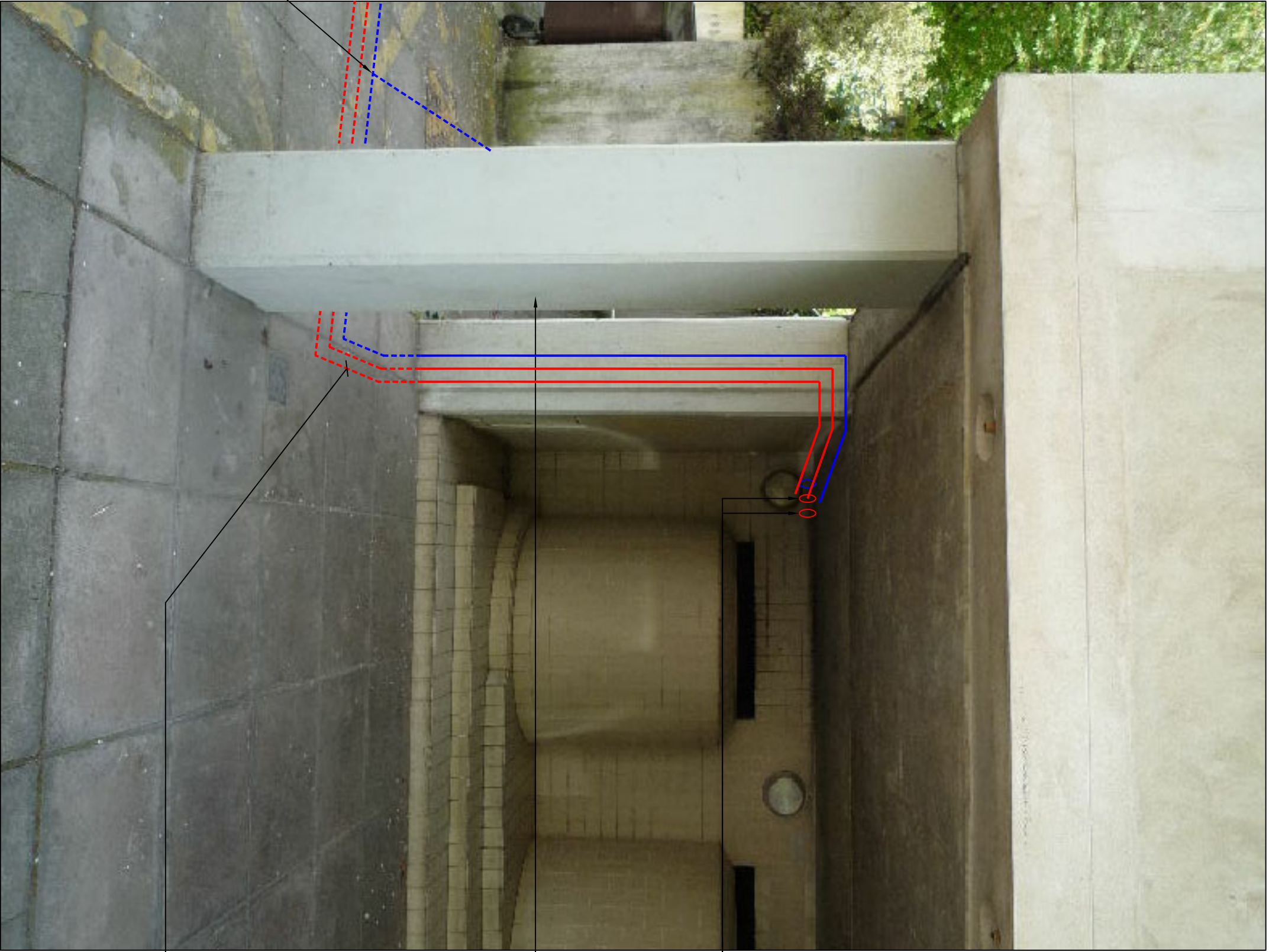
PROPOSED HTG PIPE DISTRIBUTION TO SERVE BLOCKS C2 & C1 (TYPICAL) PHOTO REF P5
