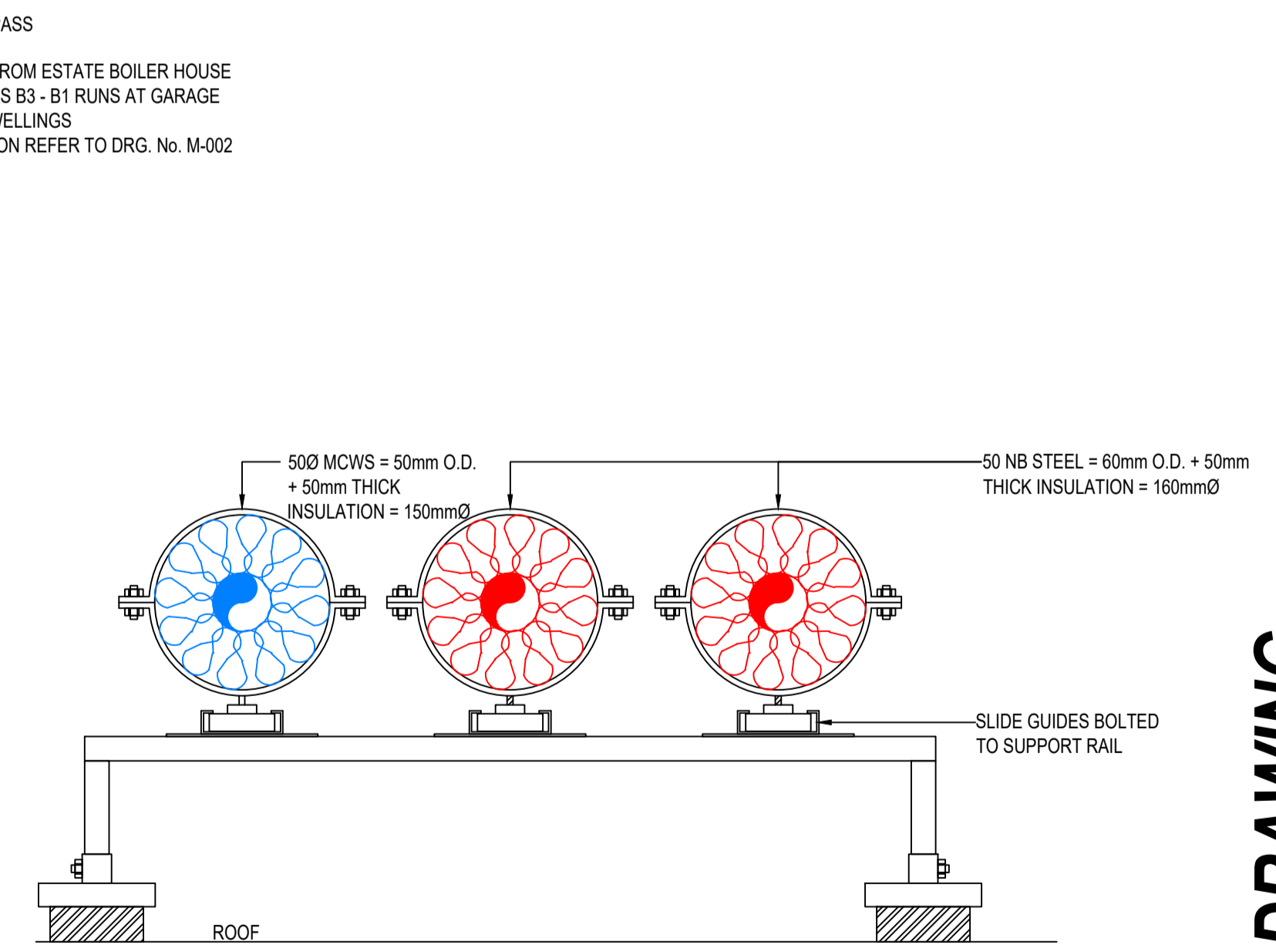
BLOCK B ROOF SUPPORTS SCALE N.T.S.
