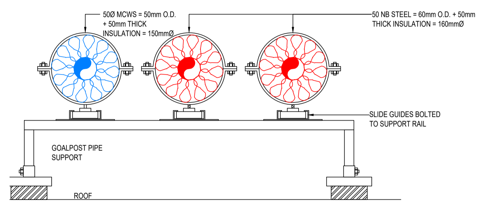
BLOCK B ROOF SUPPORTS SCALE N.T.S.
