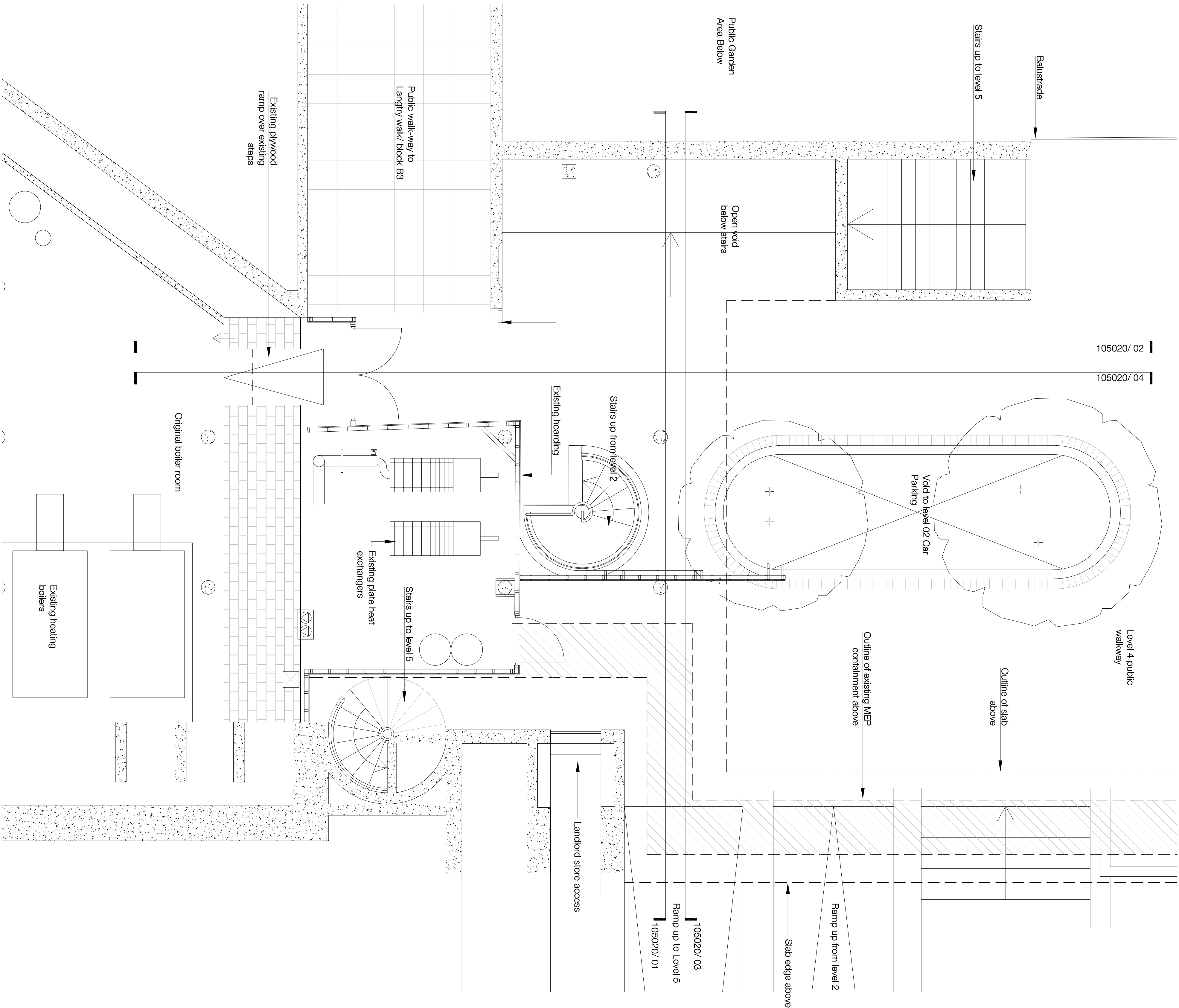
01 Existing Level 4 Combined Plan - Block B Plant Rooms 1:50
