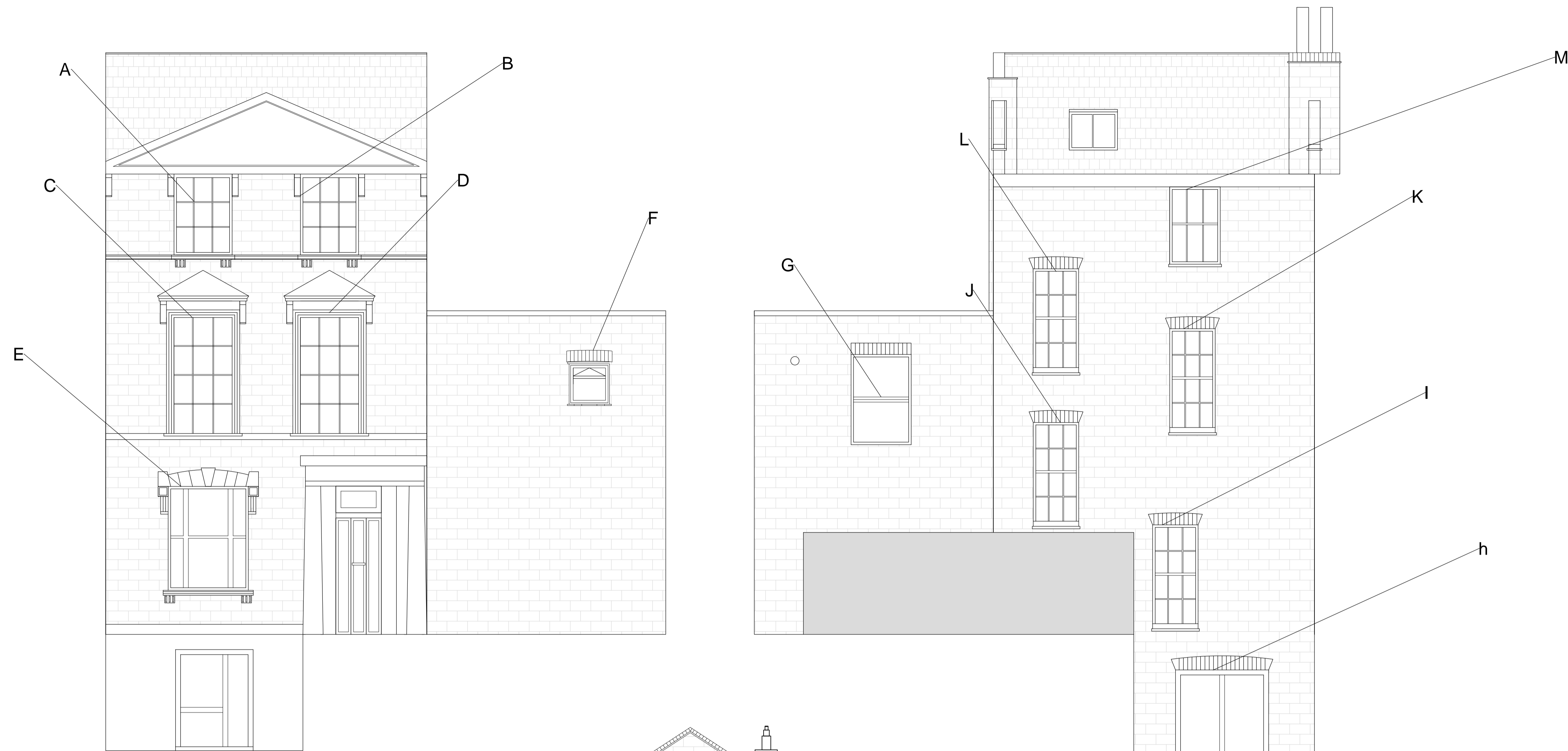
EXISTING FRONT ELEVATION
