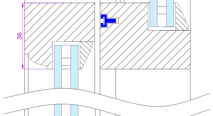
SECTION THROUGH MEETING RAIL - SCALE 1:1
