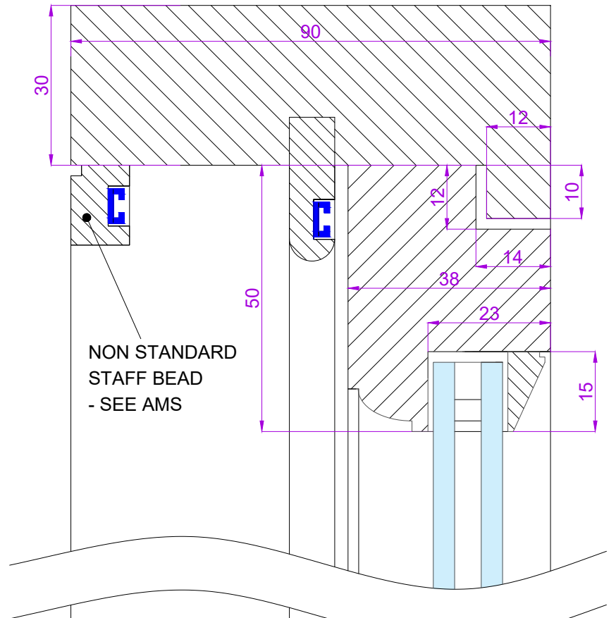
SECTION THROUGH FRAME HEAD - SCALE 1:1
