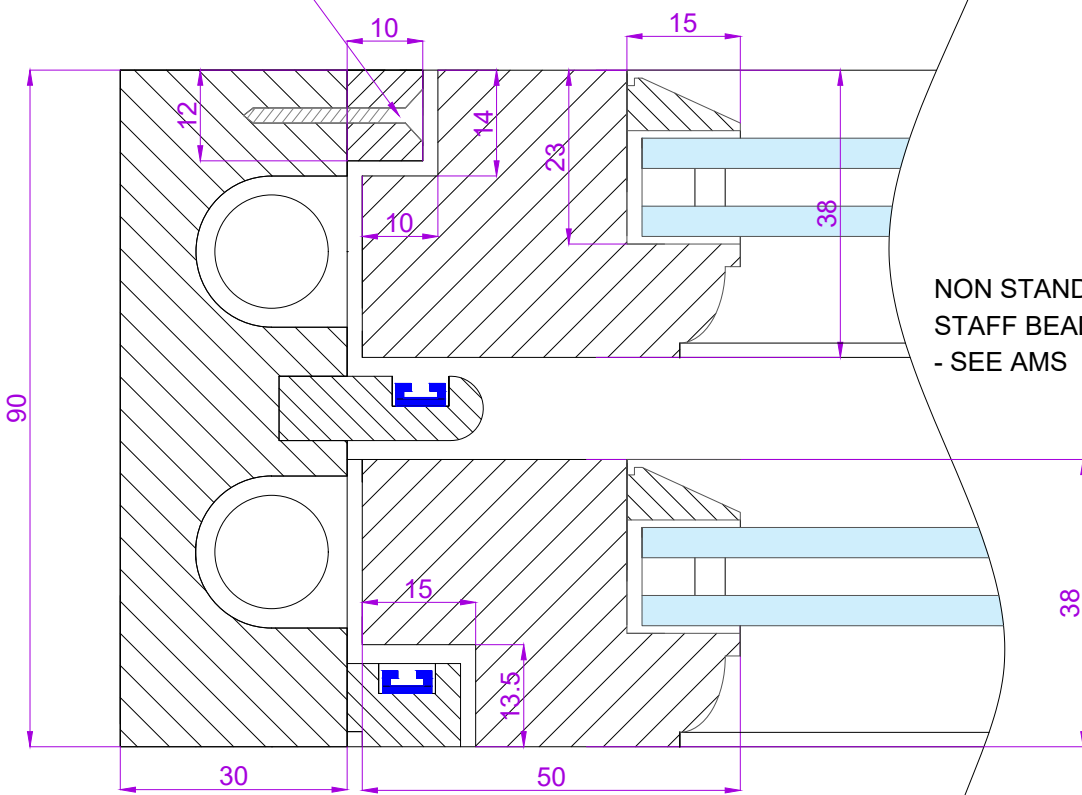
SECTION THROUGH FRAME STILE - SCALE 1:1
