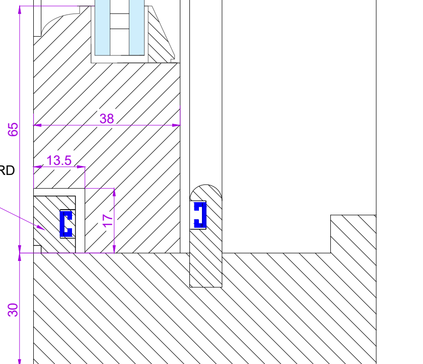
SECTION THROUGH CILL - SCALE 1:1
