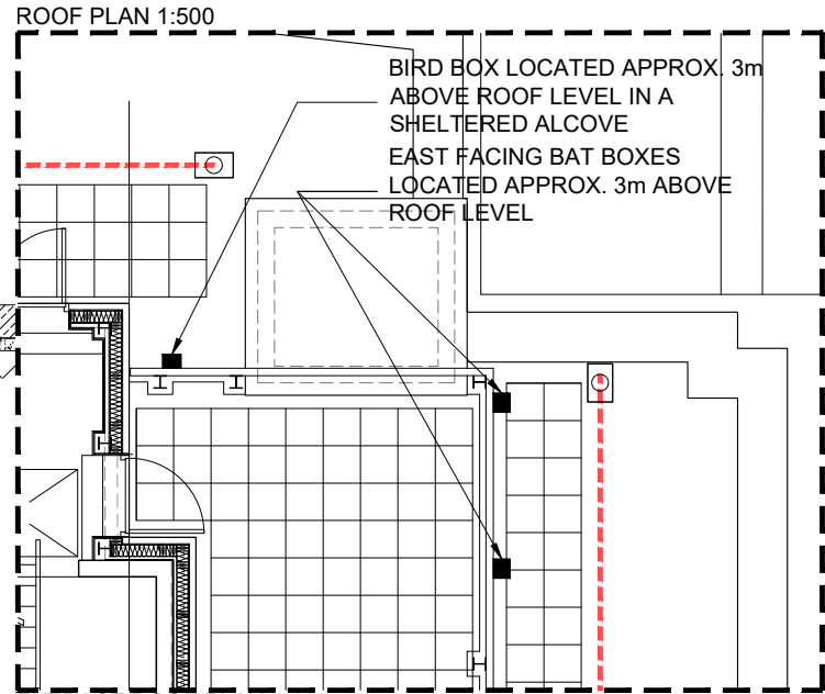
EXTRACT ROOF PLAN 1:100
