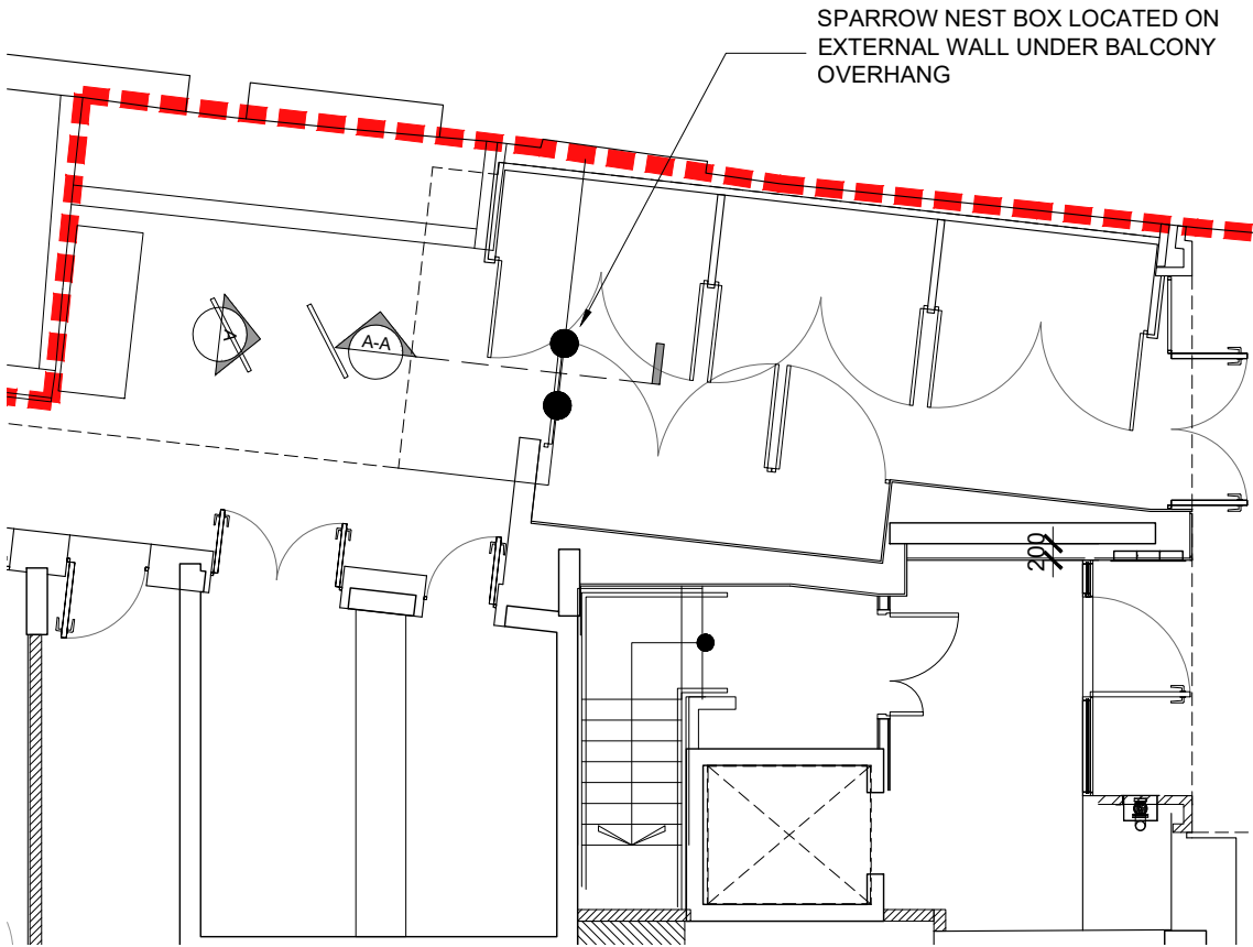
PLAN LOCATION 1:100
