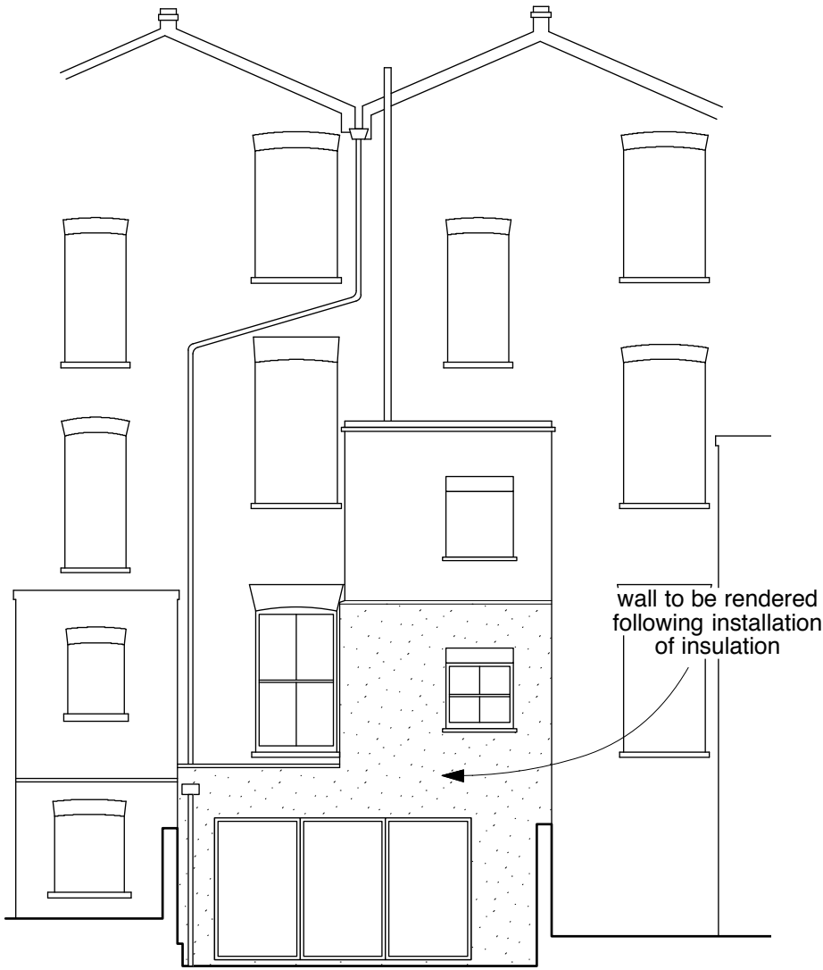
Rear Elevation
