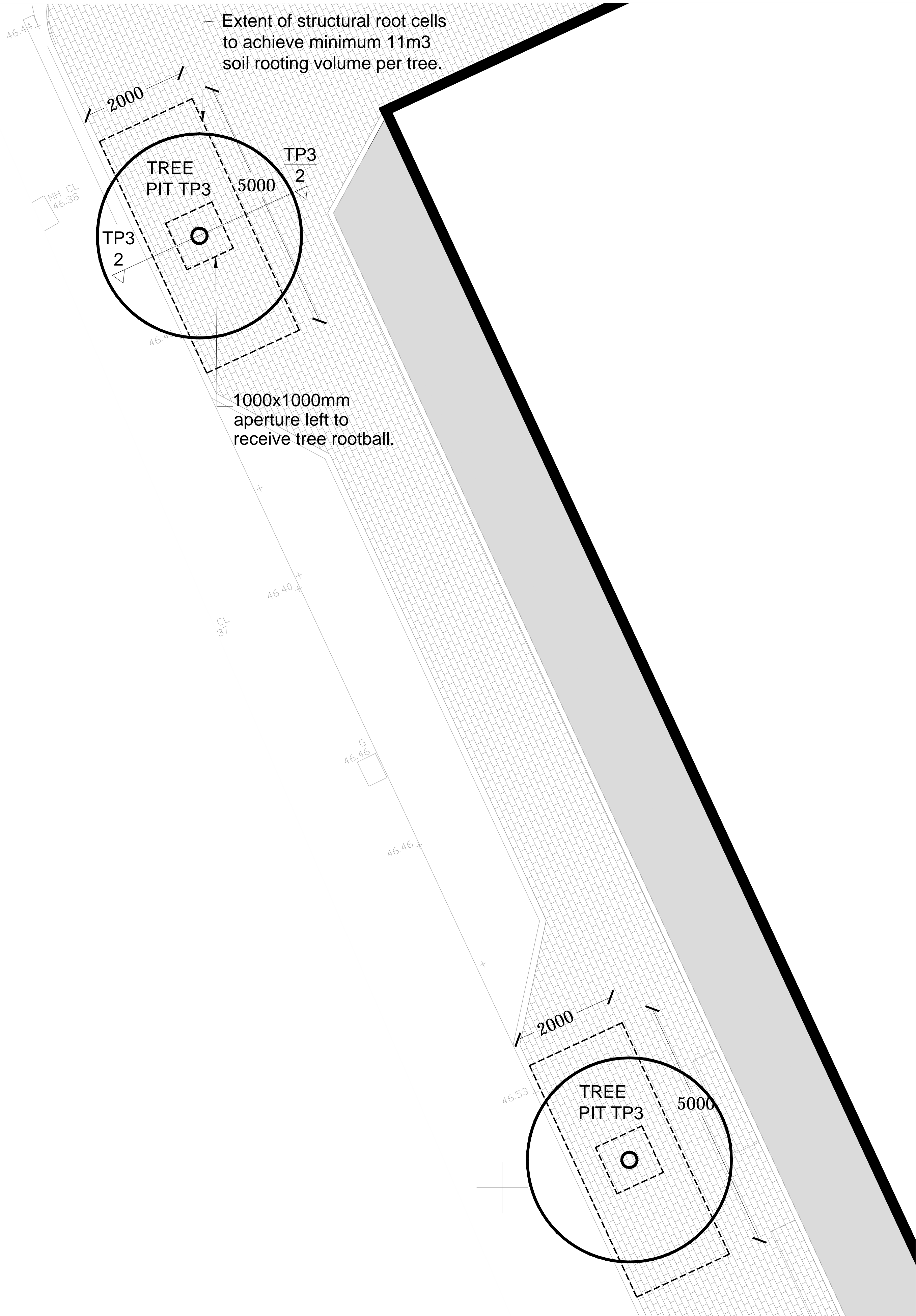
PLAN - TREE PIT IN STREET WITH HARD SURROUND & EXTENT OF CELLS SCALE 1:50@A1
