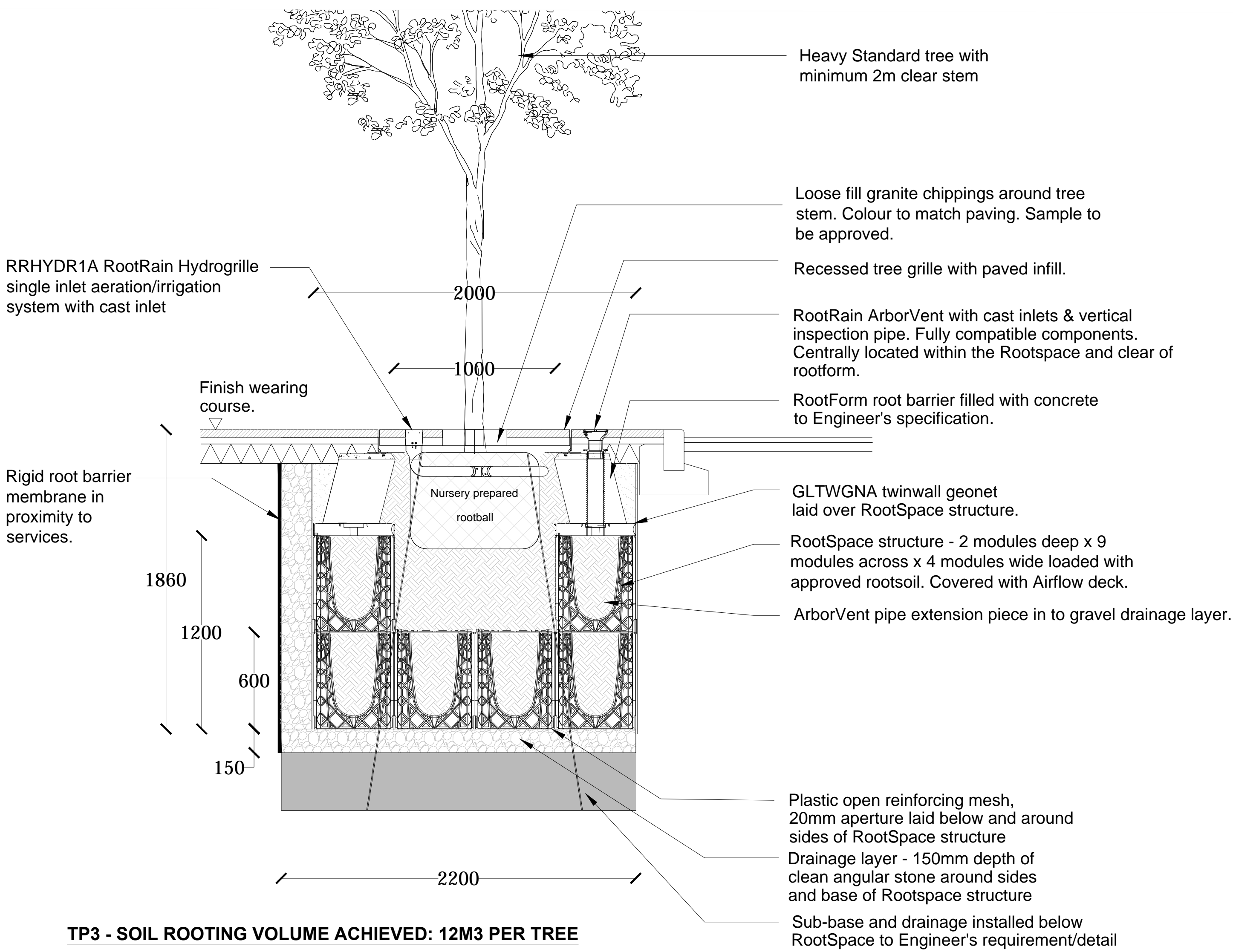
TP3 2 TREE PIT IN STREET WITH HARD SURROUND & STRUCTURAL ROOT CELLS SCALE 1:20@A1
