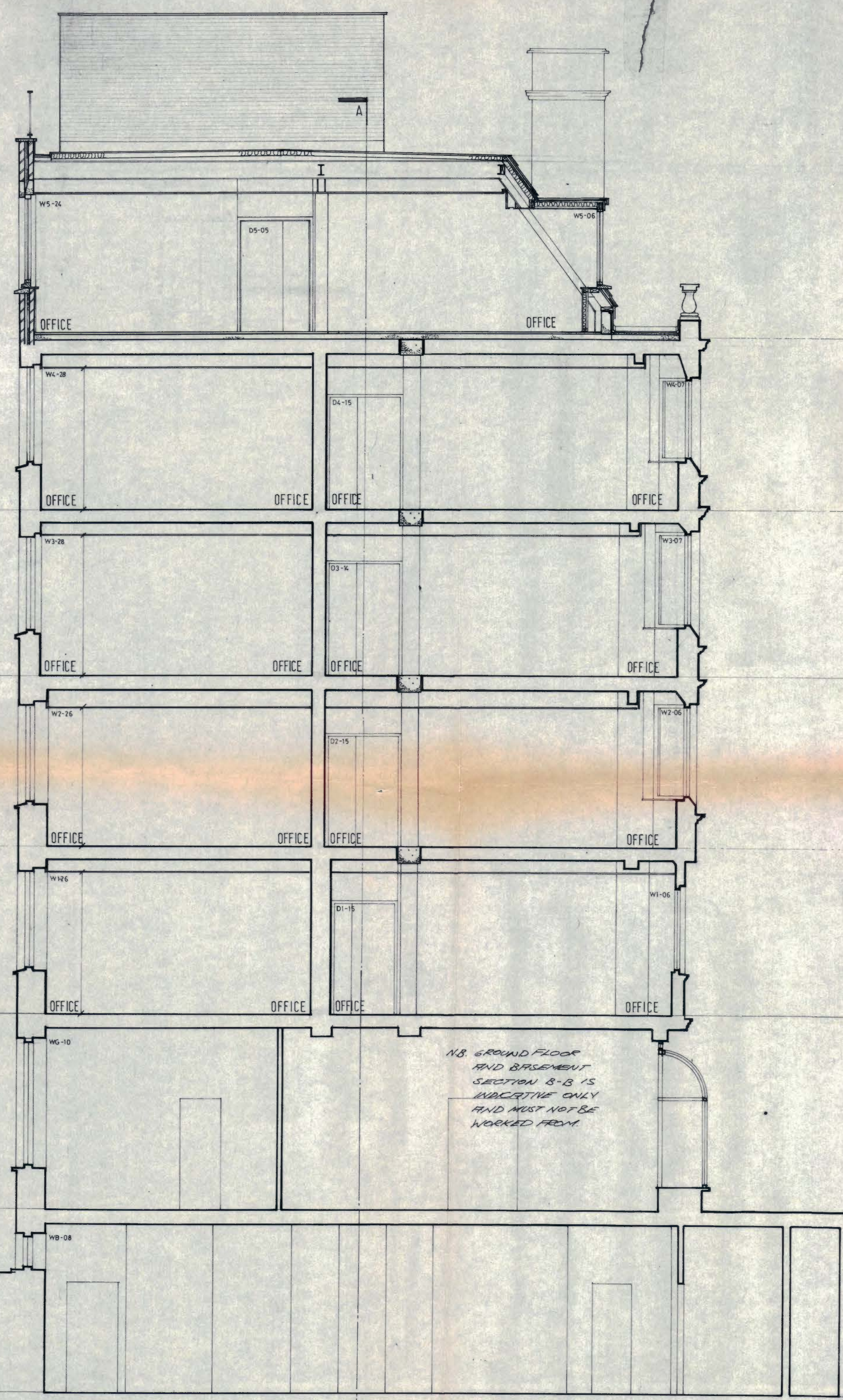
SICILIAN HOUSE _ SECTION B-B
