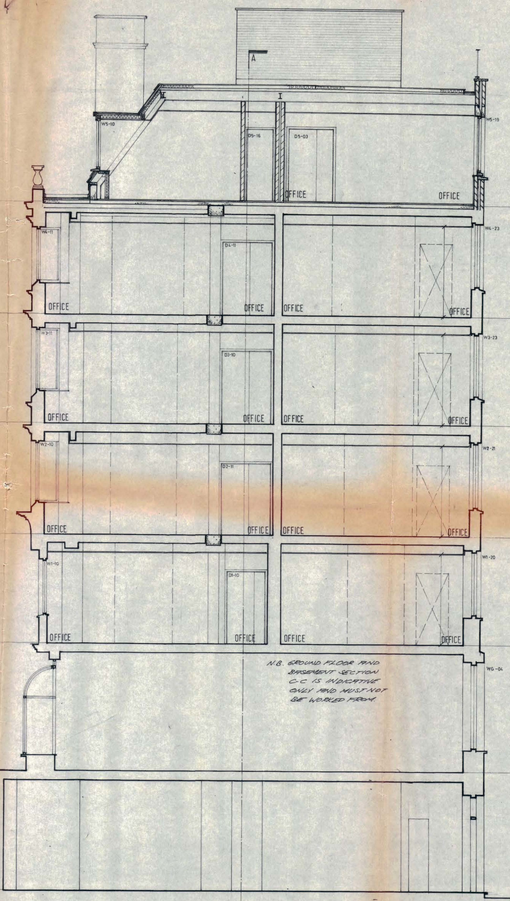
VERNON HOUSE _ SECTION C-C
