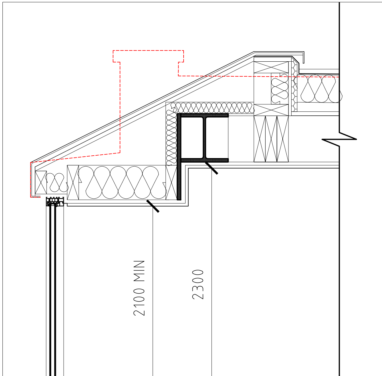
SK.01 THIRD FLOOR PARAPET DETAIL SKETCH 02.06.2020
