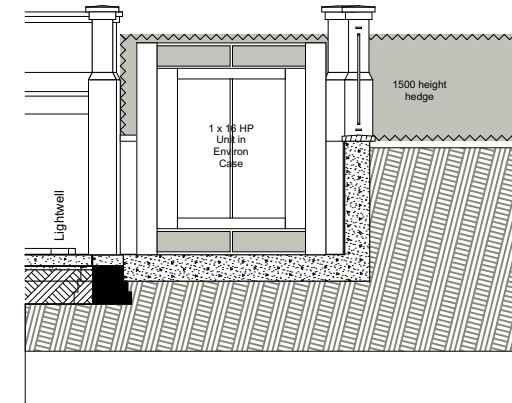
Section 1:100@A3
