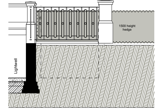
Elevation 1:100@A3
