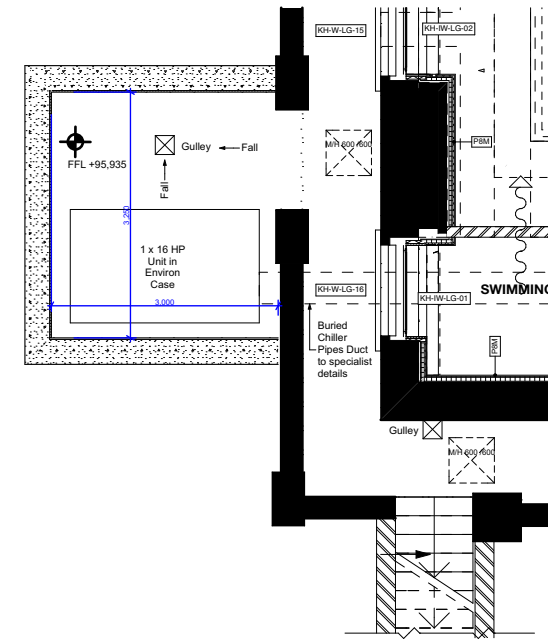
Lower Ground Floor Plan 1:100@A3
