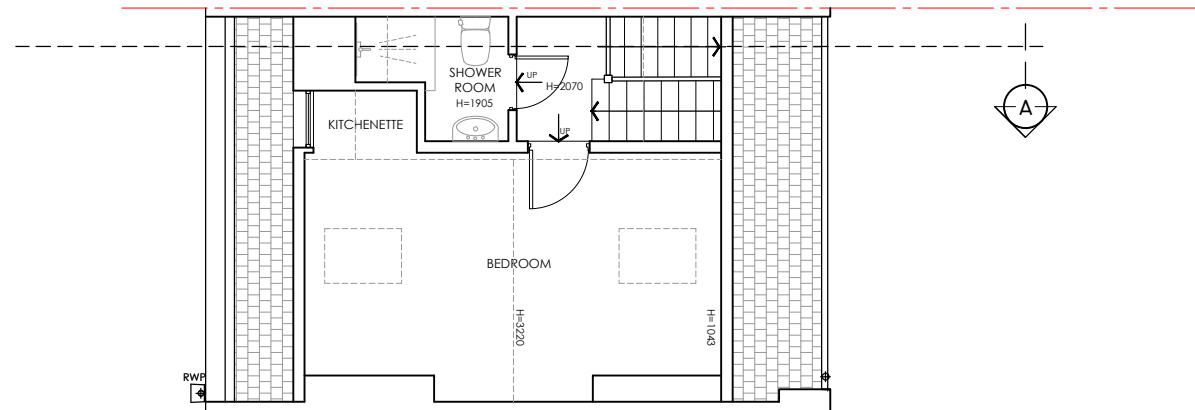
EXISTING LOFT FLOOR PLAN
