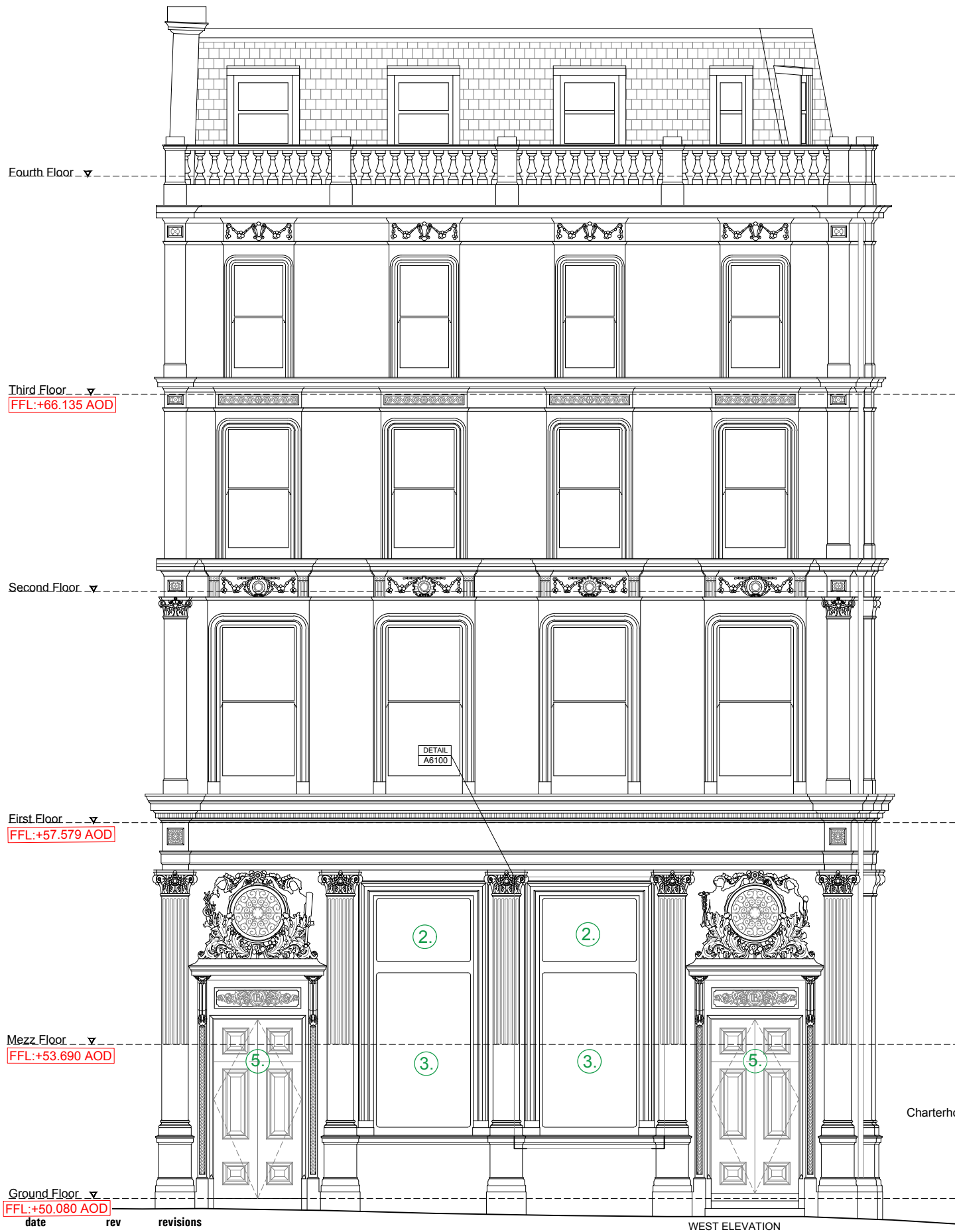
WEST ELEVATION
