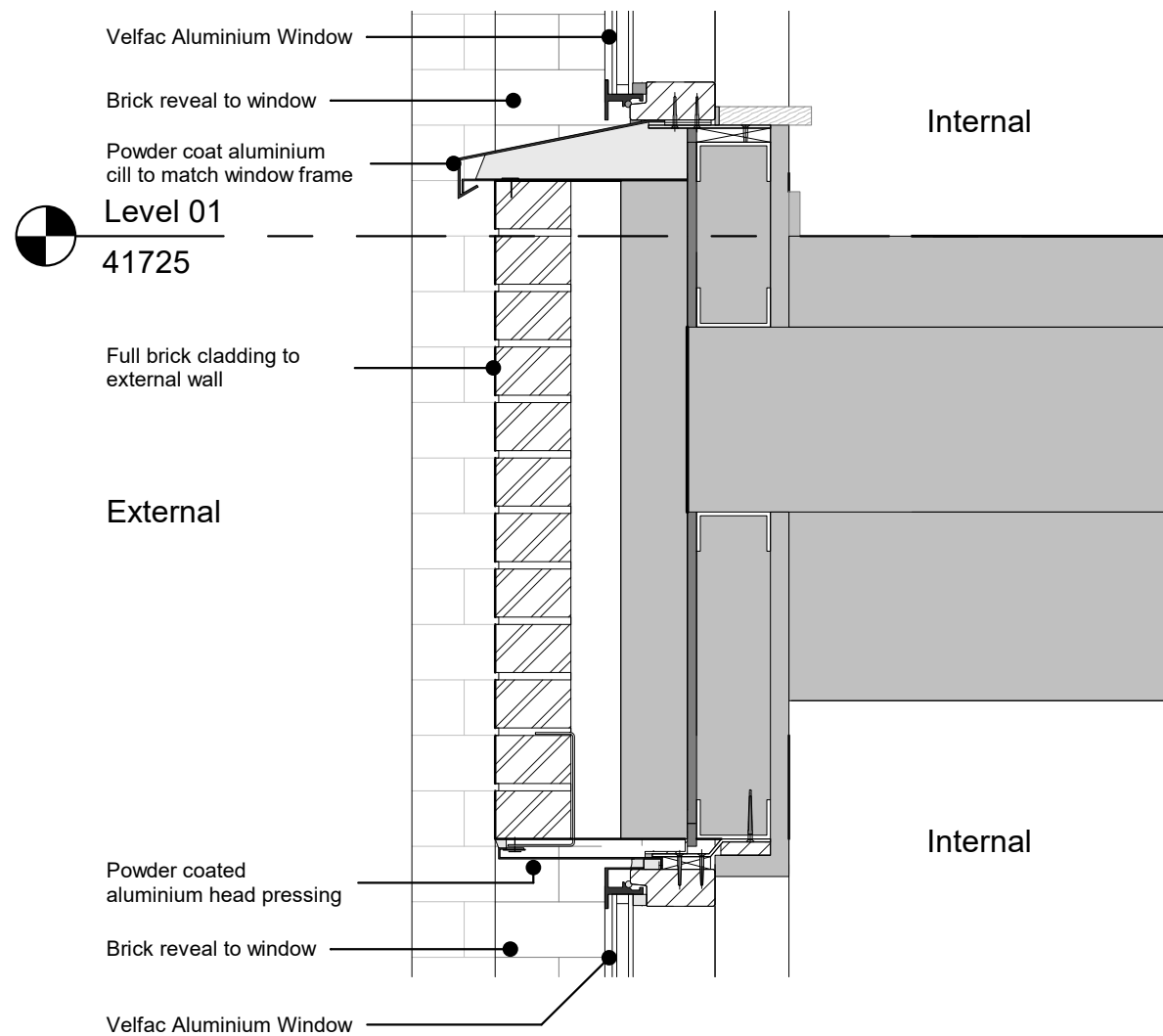
1 | Window Head and Cill Detail in Brick Wall Scale 1 : 10
