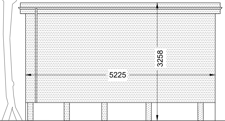
Rear Elevation
