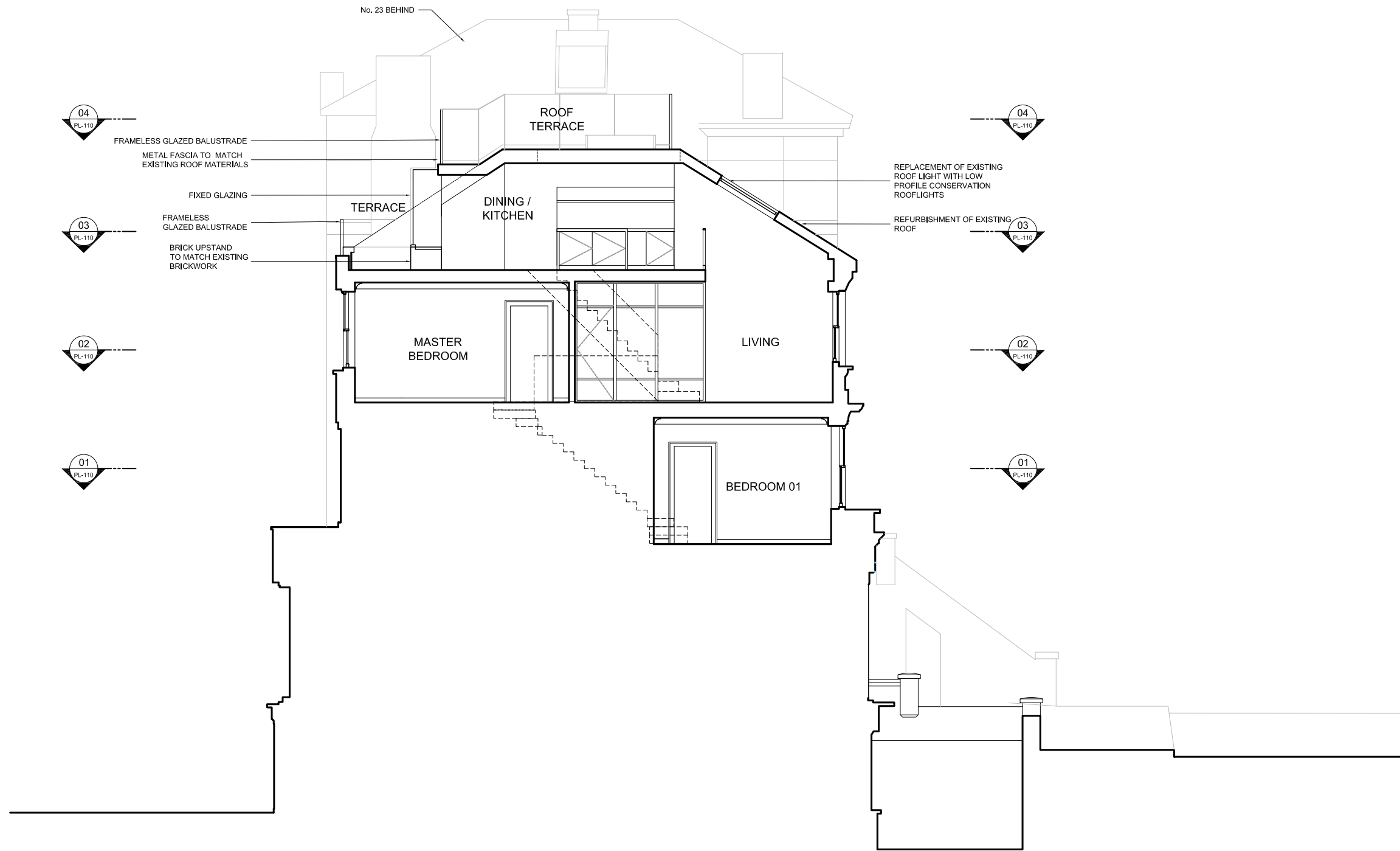
PROPOSED SECTION AA SCALE 1:100 @ A3
