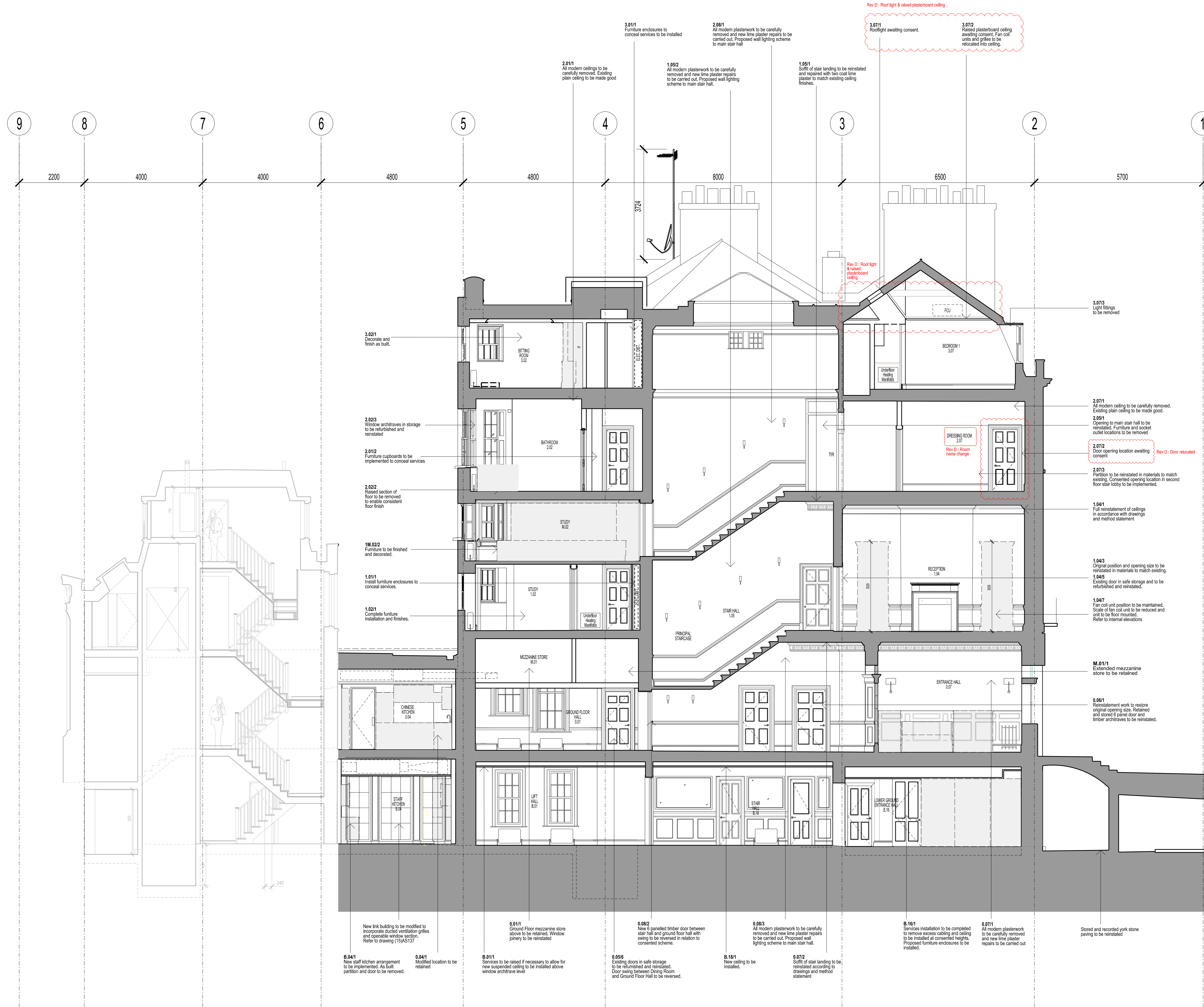
SECTION H - H
