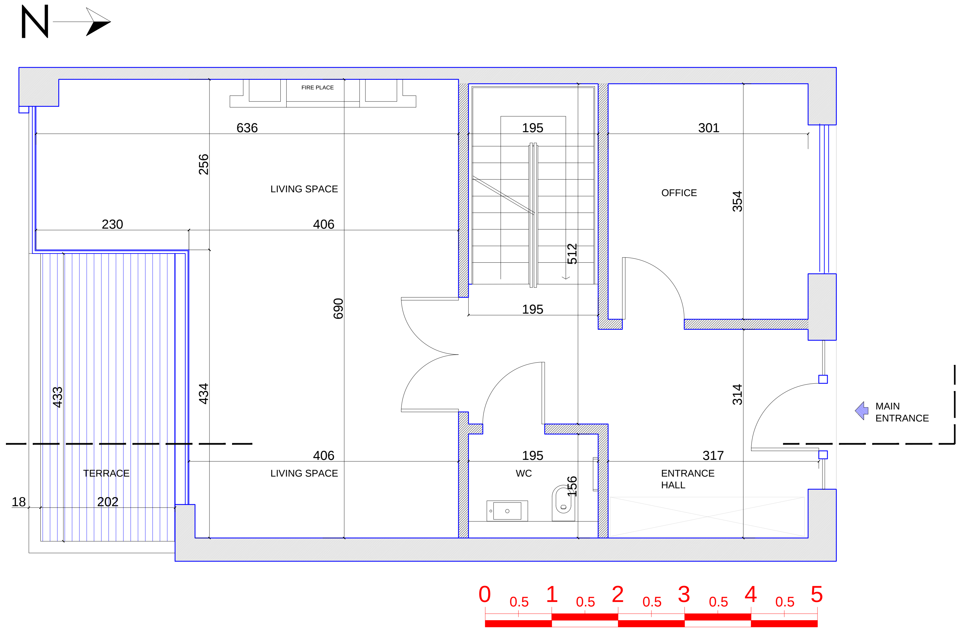
GROUND FLOOR
