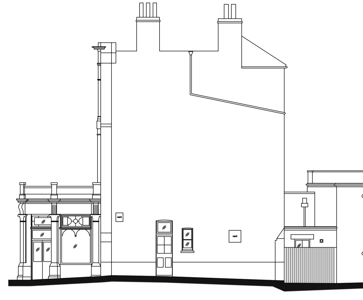
SIDE ELEVATION B - B
