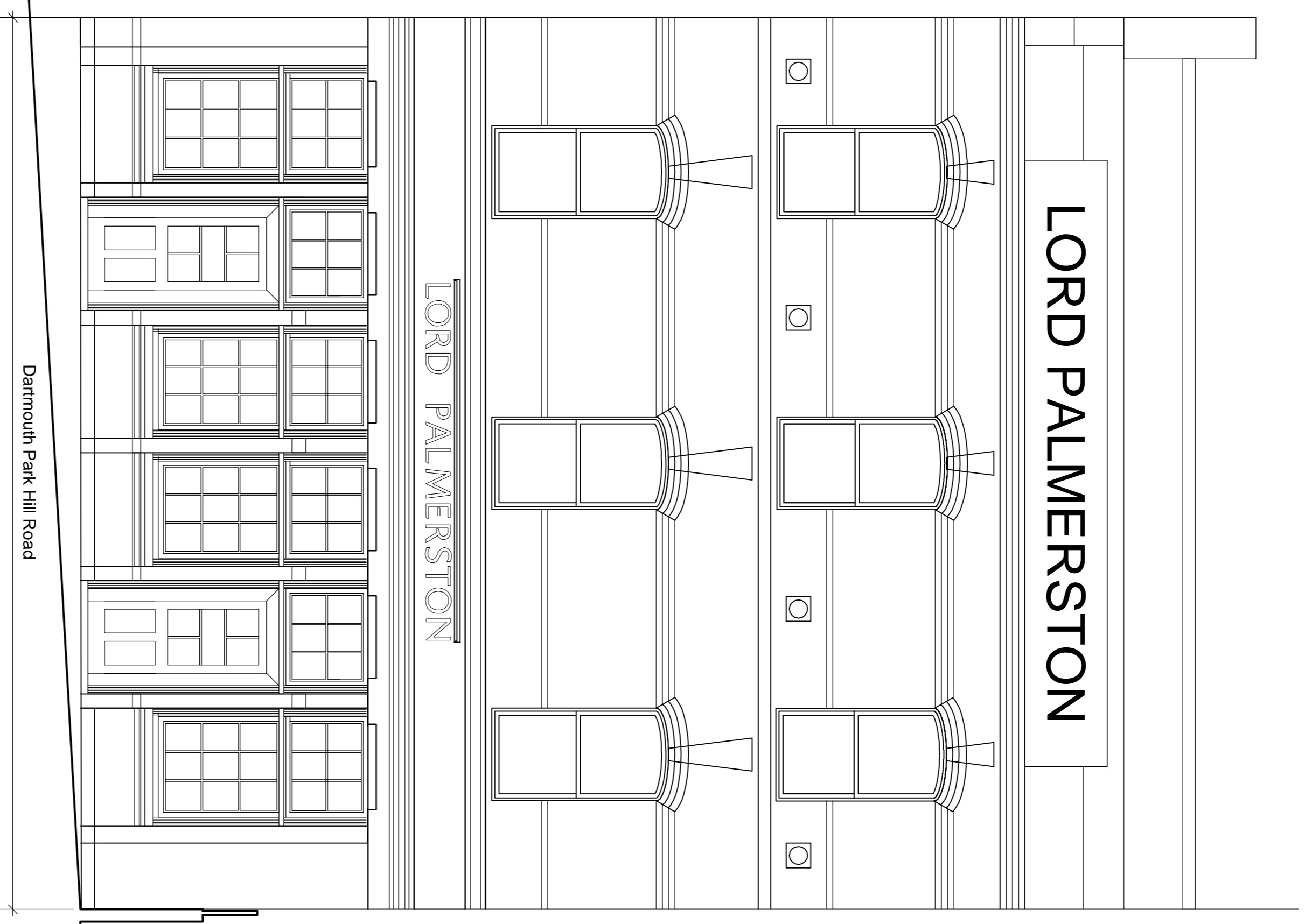
1 PROPOSED FRONT EAST FACING ELEVATION
