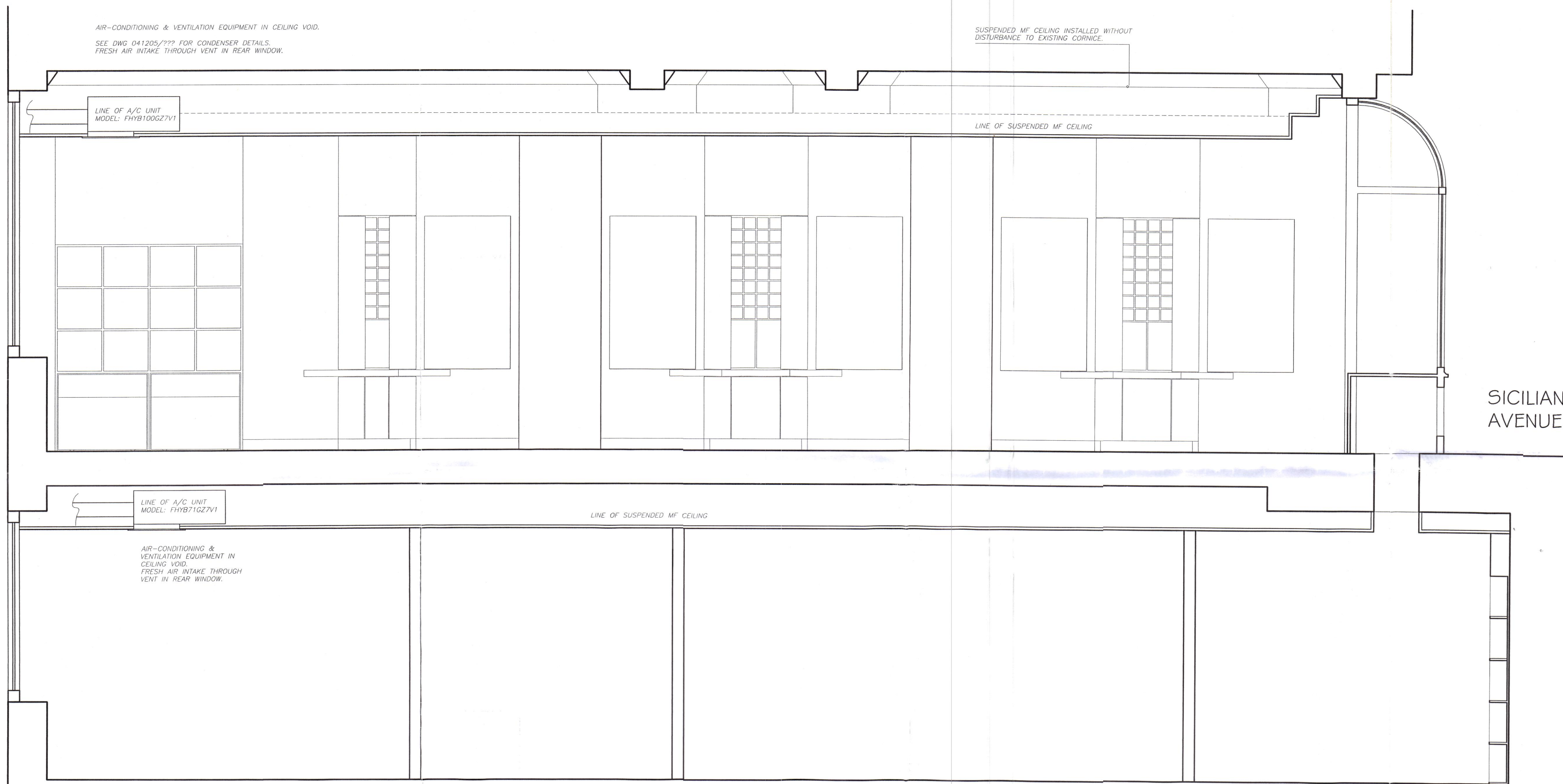
PROPOSED SECTION BB THROUGH UNIT 15
