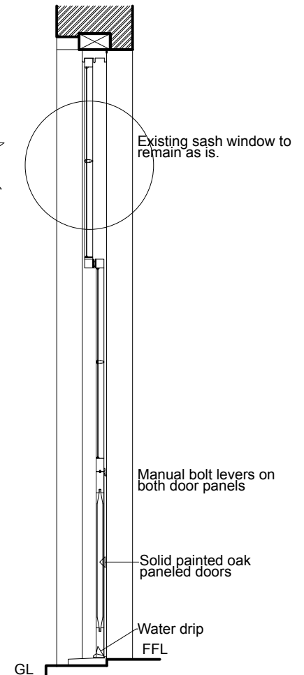
Sash Window Section Sc. 1:25
