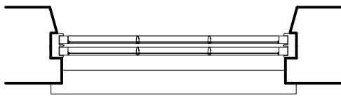
Sash Window Upper Plan Sc. 1:25
