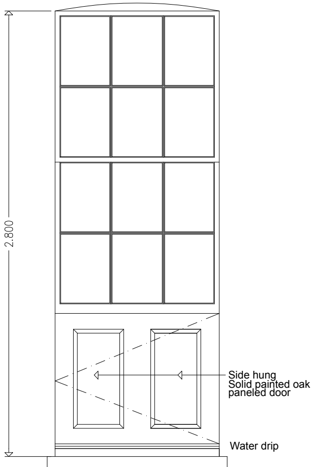
Sash Window Elevation Sc. 1:25
