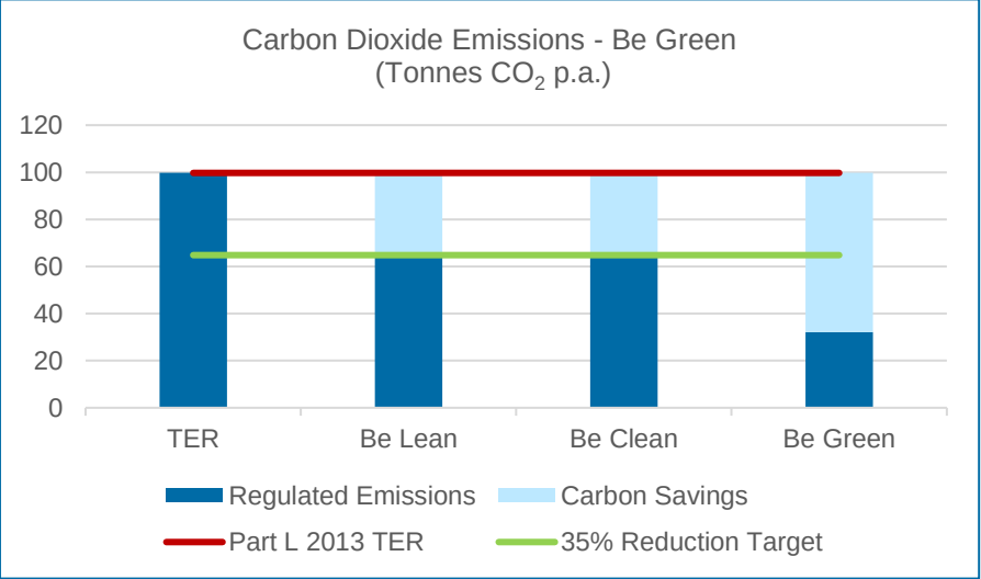
Figure 14: Regulated carbon dioxide emissions from each stage of the energy hierarchy for the development
