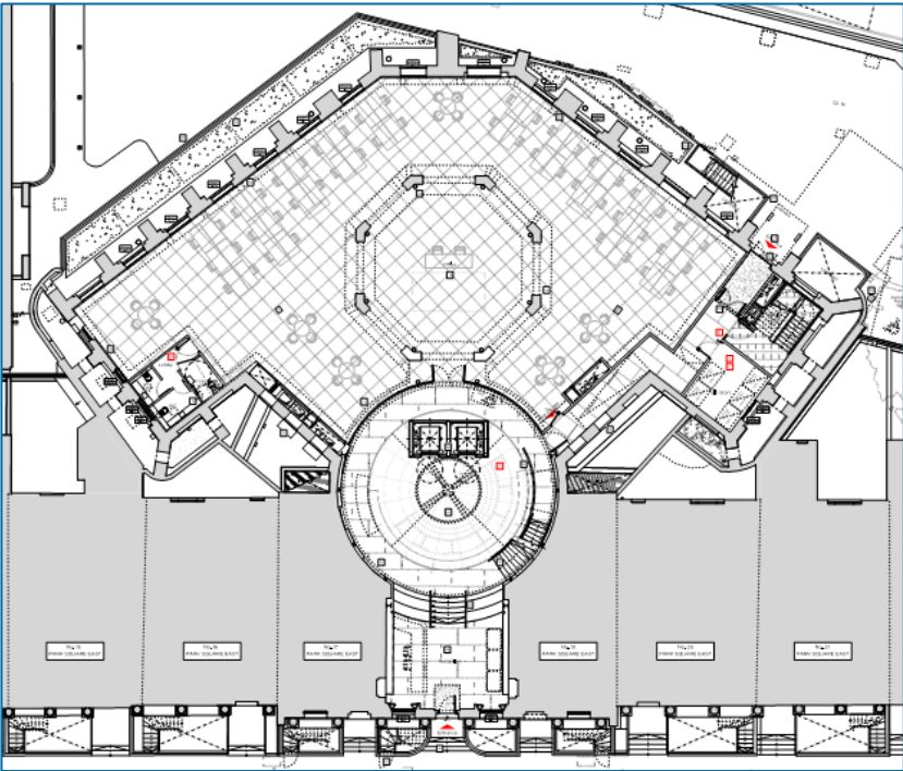
Figure 5: Proposed ground floor refurbishment
