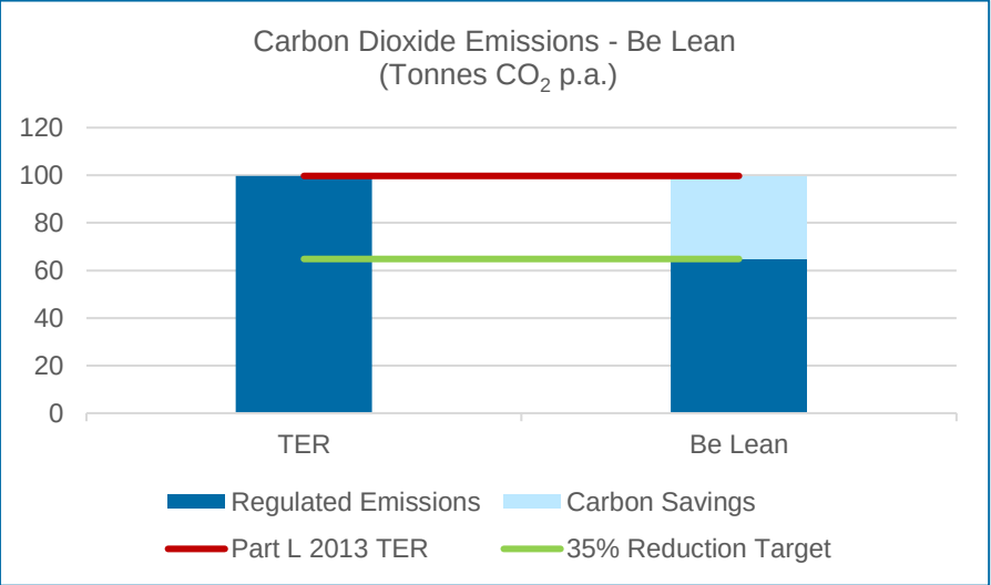
Figure 10: Be Lean' Regulated Carbon Dioxide emissions for the development
