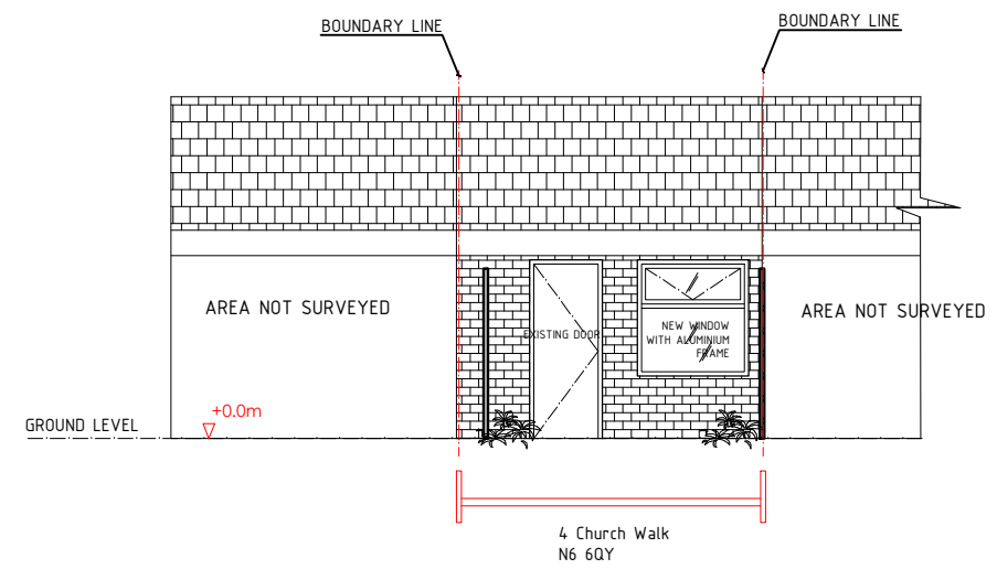
GARAGE-NORTH-WEST-ELEVATION-AS-PROPOSED
