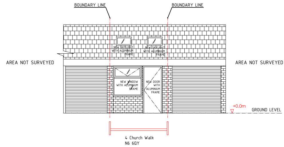
GARAGE-SOUTH-EAST-ELEVATION-AS-PROPOSED
