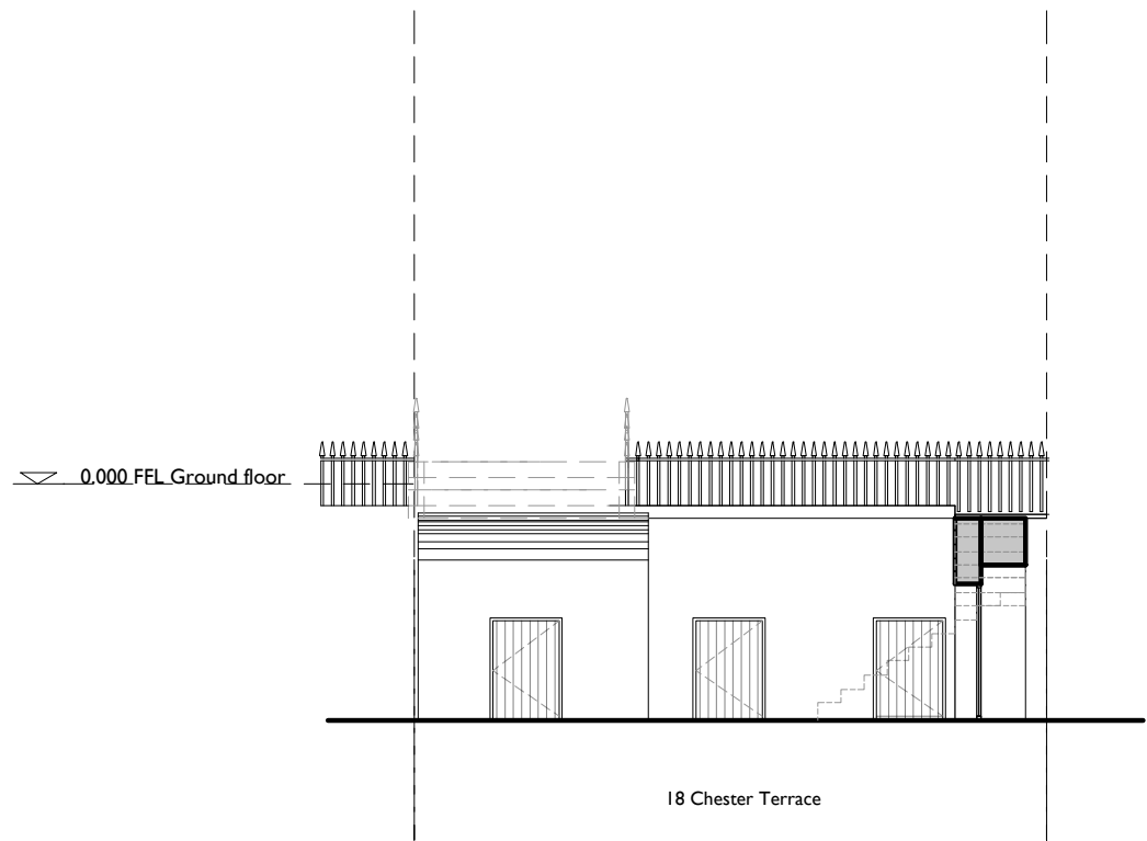
01 External staircase
