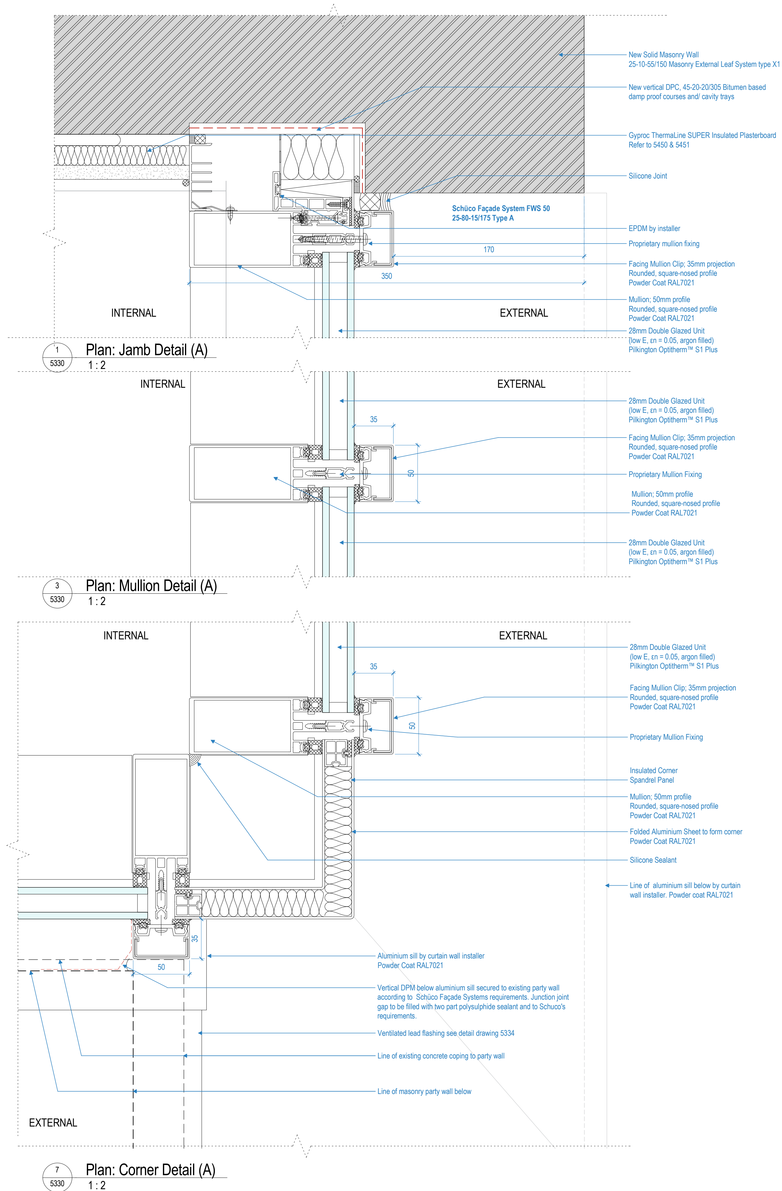
Curtain Wall Type A 25-80-15/175 Type A
