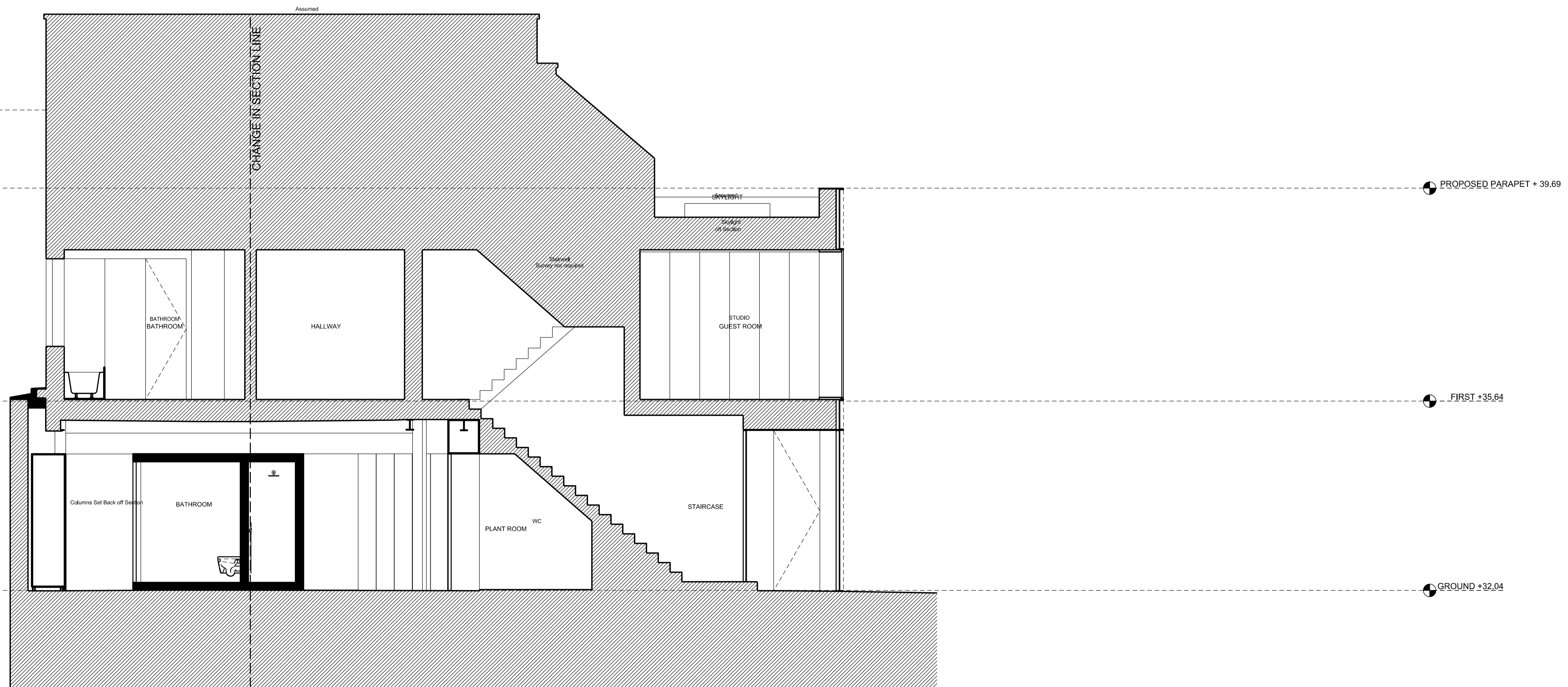
EXISTING SECTION Y3
