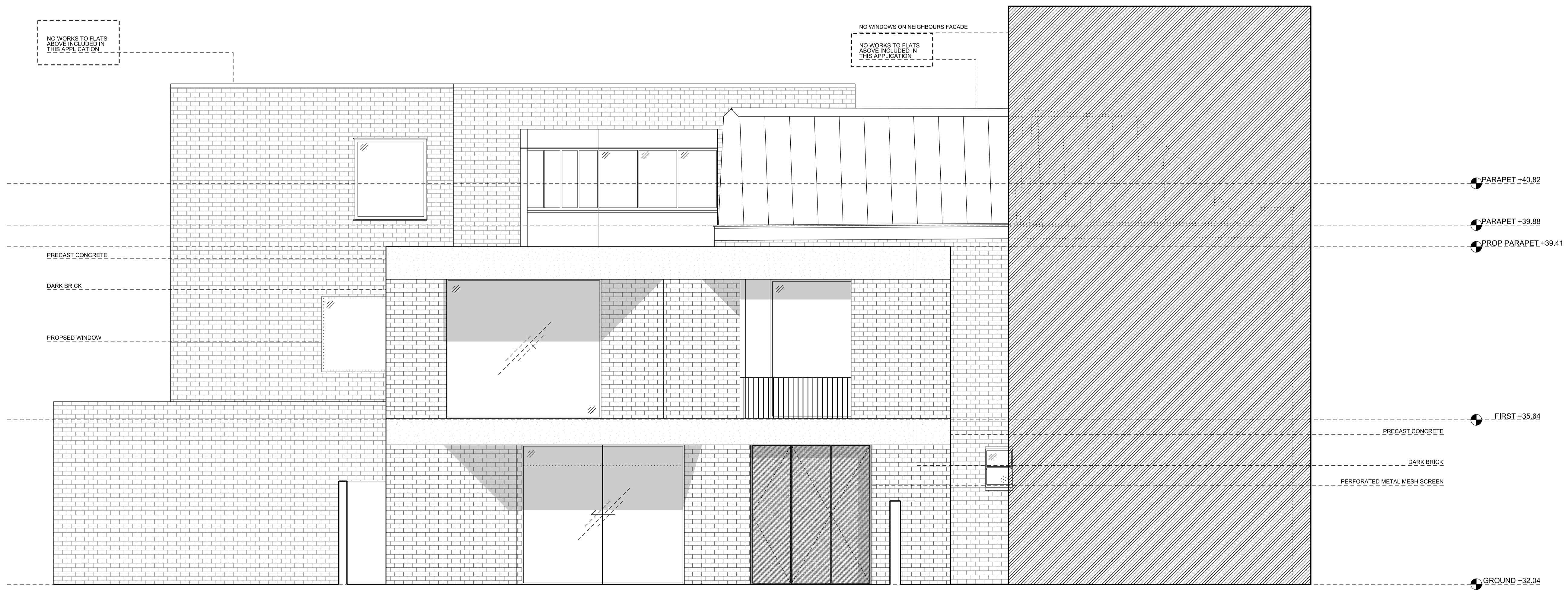
PROPOSED SECTION Y1
