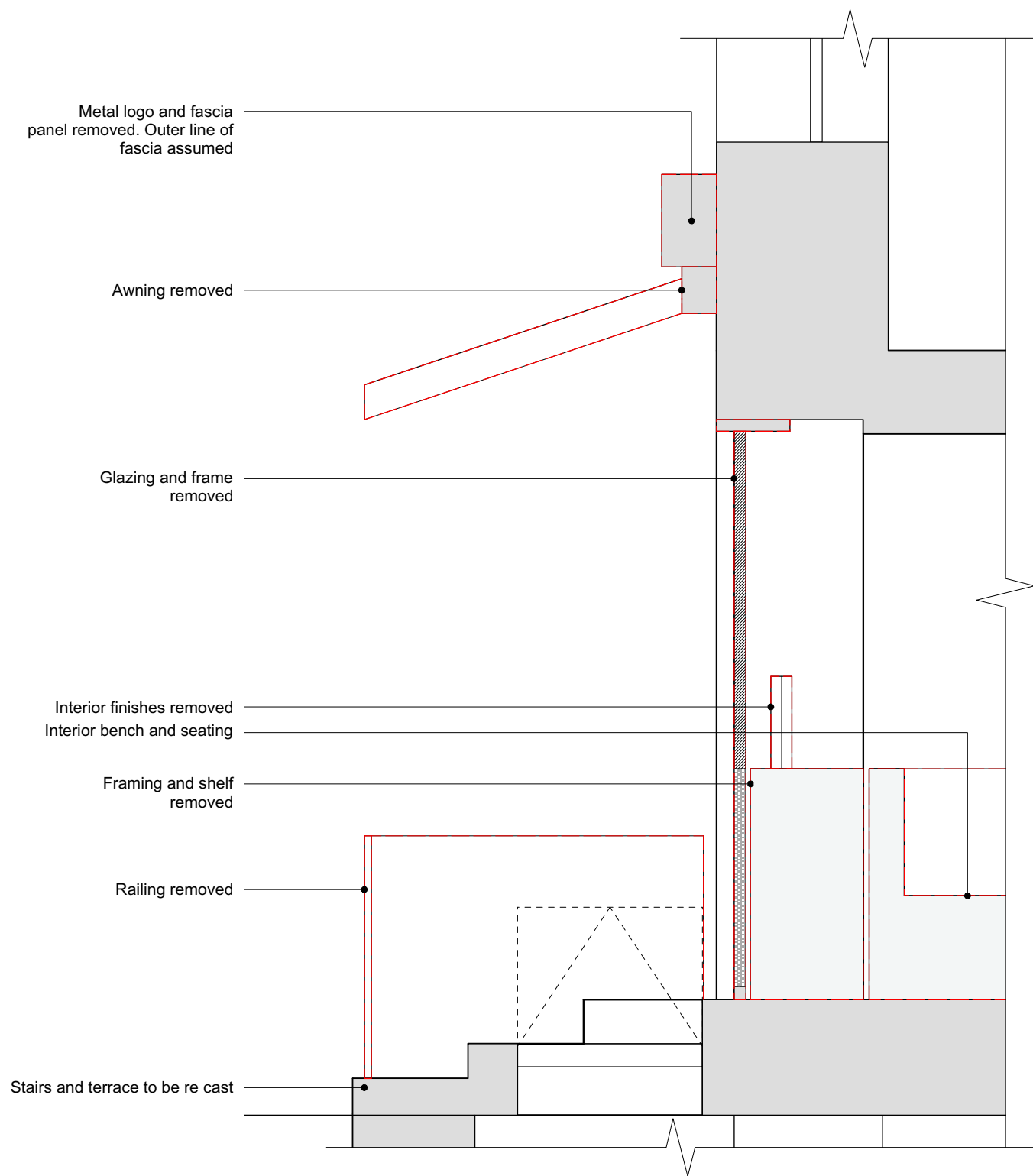
1 EXISTING DETAILED SECTION A 1:25
