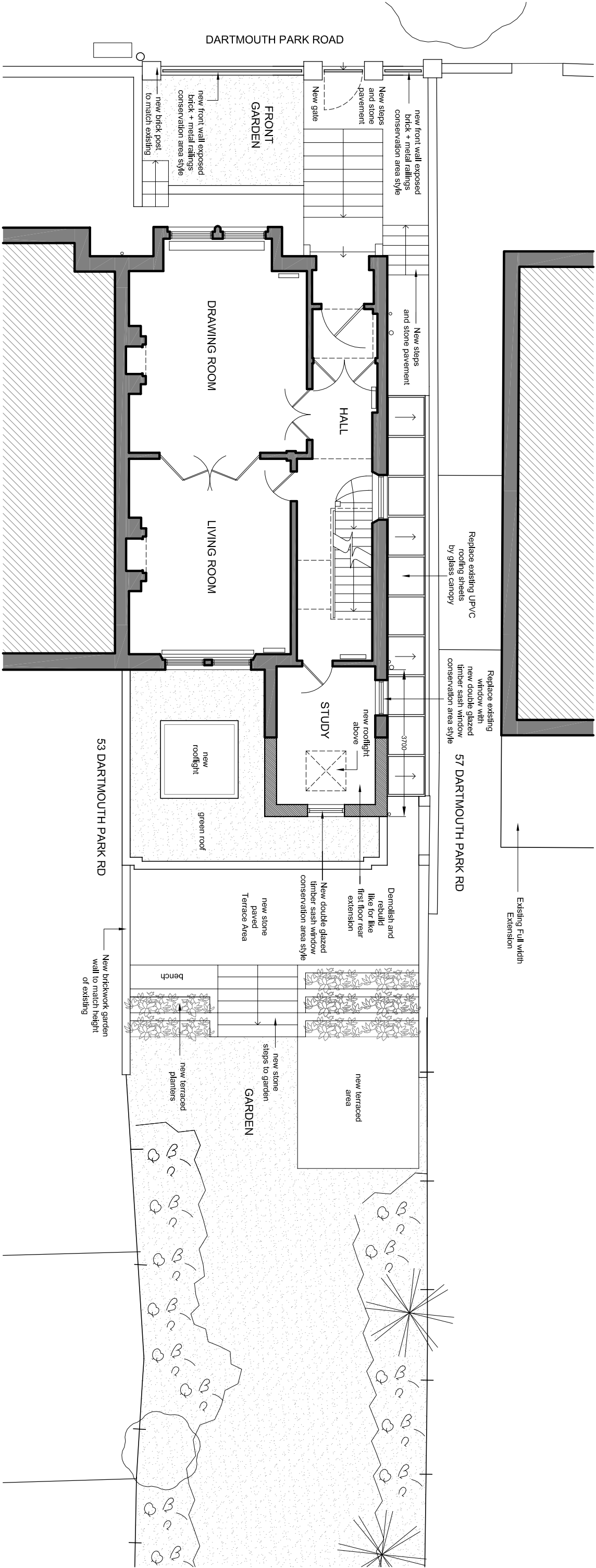
PROPOSED - Ground Floor Plan Scale 1:100@A3 PA-02
