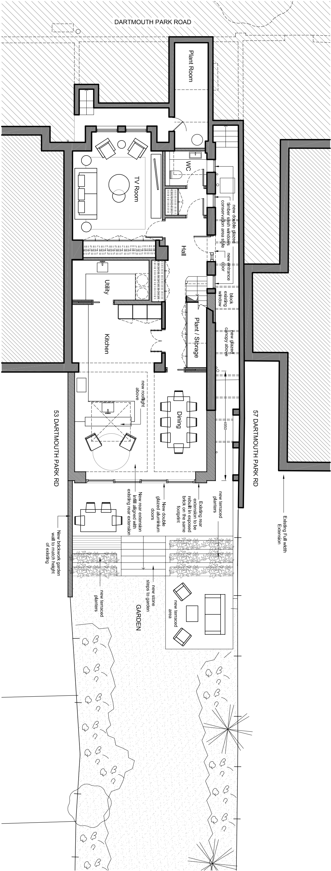
PROPOSED - Lower Ground Floor Plan Scale 1:100@A3 PA-01
