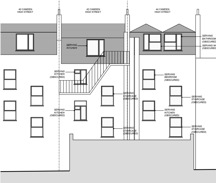
3 SK-001 EXISTING ELEVATION C REAR ELEVATION TO 42 & 44 CAMDEN HIGH STREET SCALE@A1 1:100 SCALE@A3 1:200
