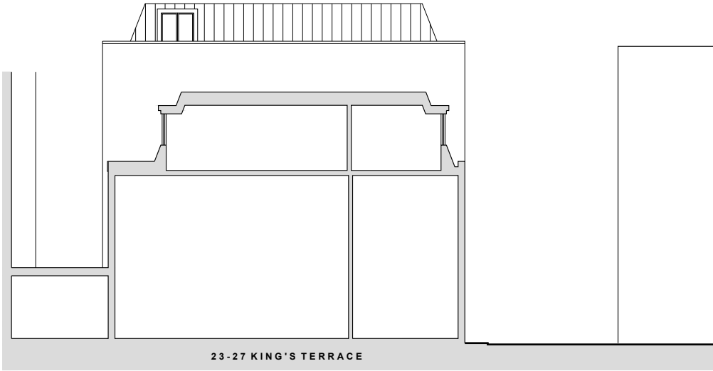
5 SK-001 EXISTING SECTION SCALE@A1 1:100 SCALE@A3 1:200
