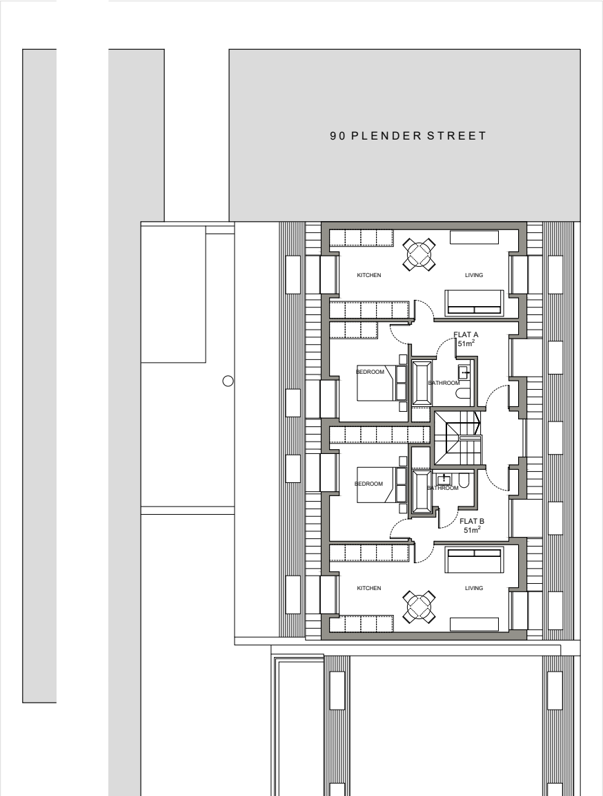
2 PROPOSED THIRD FLOOR PLAN SK-002 SCALE@A1 1:100 SCALE@A3 1:200
