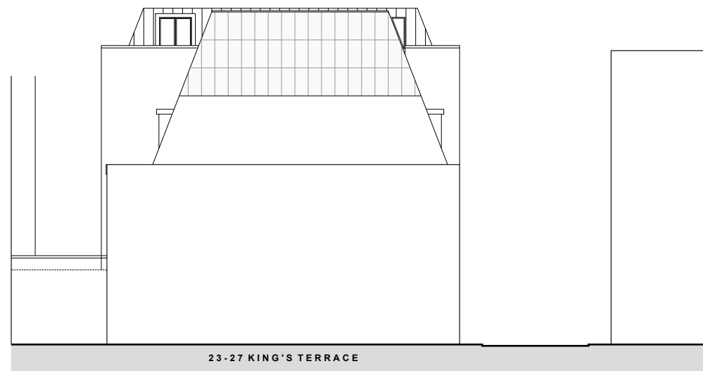
3 SK-003 PROPOSED SOUTH ELEVATION SCALE@A1 1:100 SCALE@A3 1:200
