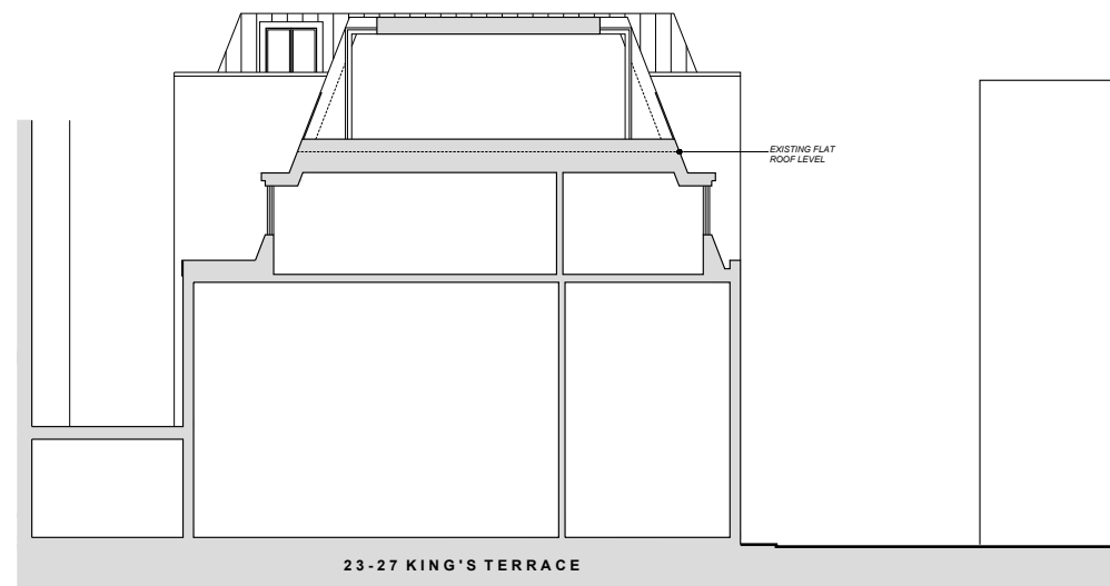
4 SK-003 PROPOSED SECTION SCALE@A1 1:100 SCALE@A3 1:200
