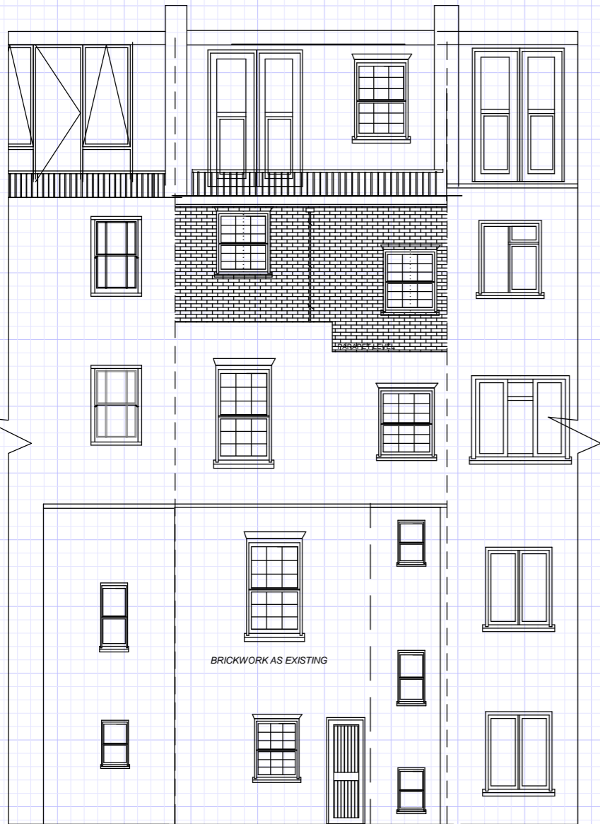
REAR ELEVATION AS PROPOSED
