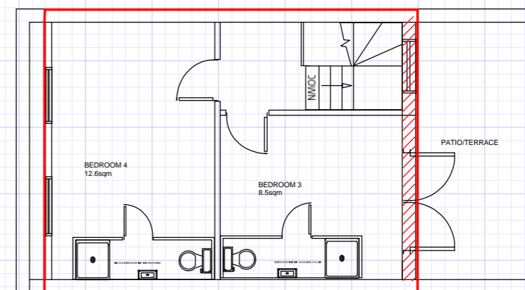
MANSARD FLOOR LEVEL-AS PROPOSED
