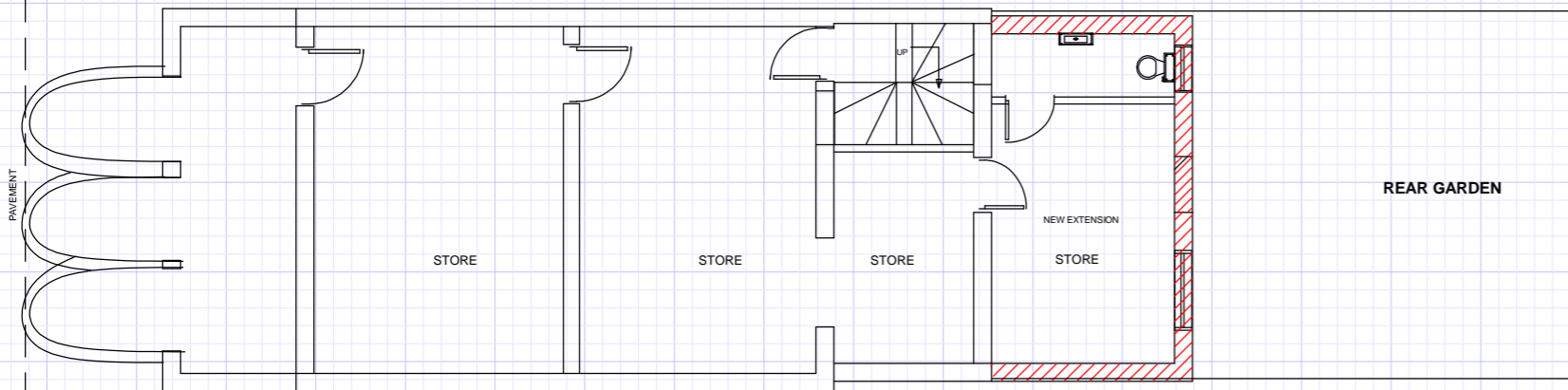
LOWER GROUND FLOOR PLAN-PROPOSED
