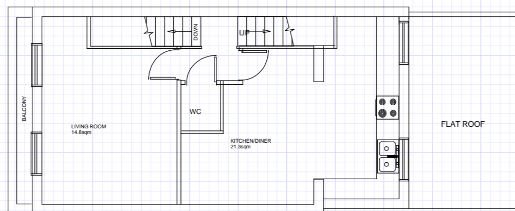
FIRST FLOOR PLAN -AS PROPOSED
