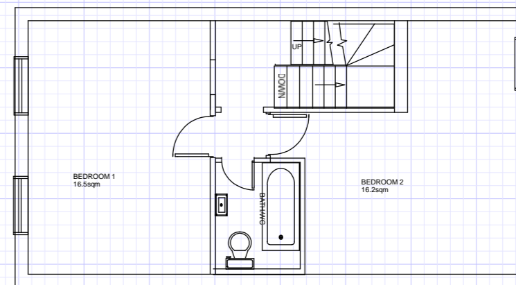
SECOND FLOOR PLAN -AS PROPOSED
