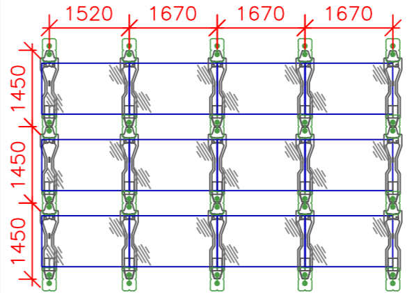
Grid Arrangement 1:100
