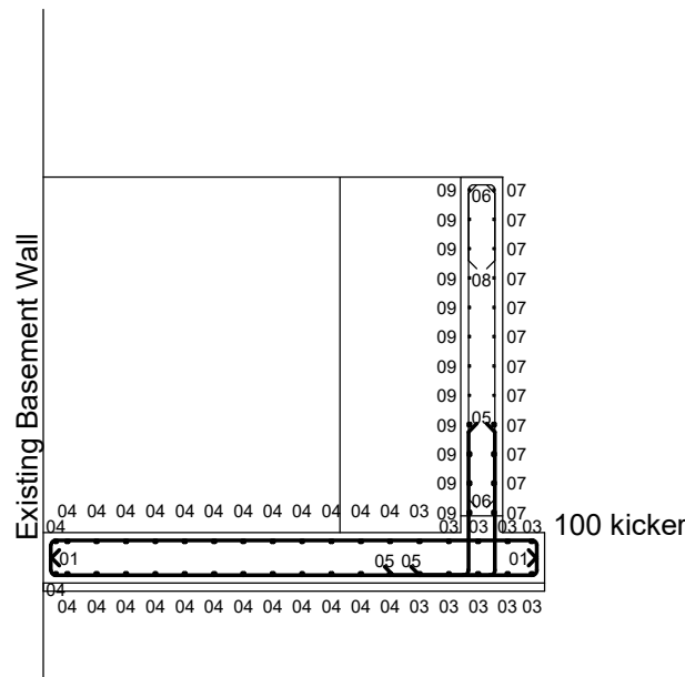
Section A-A (wall reinforcement omitted for clarity)
