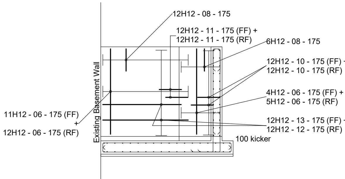
Elevation A-A (base reinforcement omitted for clarity)
