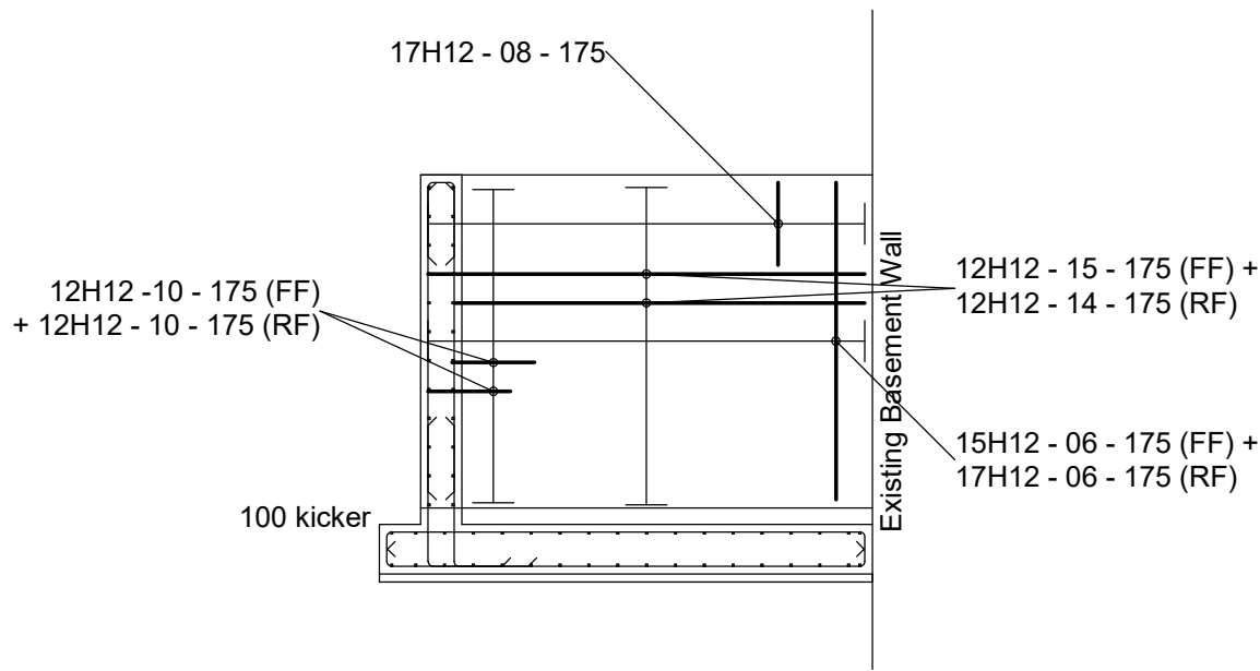
Elevation D-D (base reinforcement omitted for clarity)
