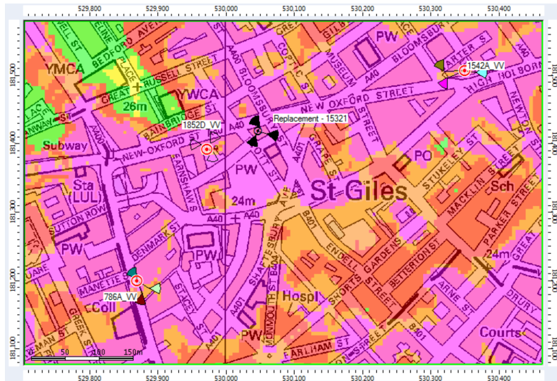
Fig. 6: Proposed LTE2100MHz, (replacement site 15321)
