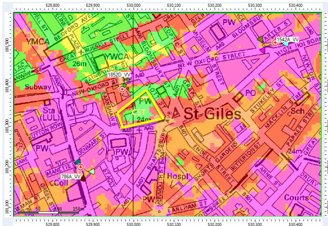
Fig. 5: Existing LTE2100MHz, (decommissioned site 1852)
