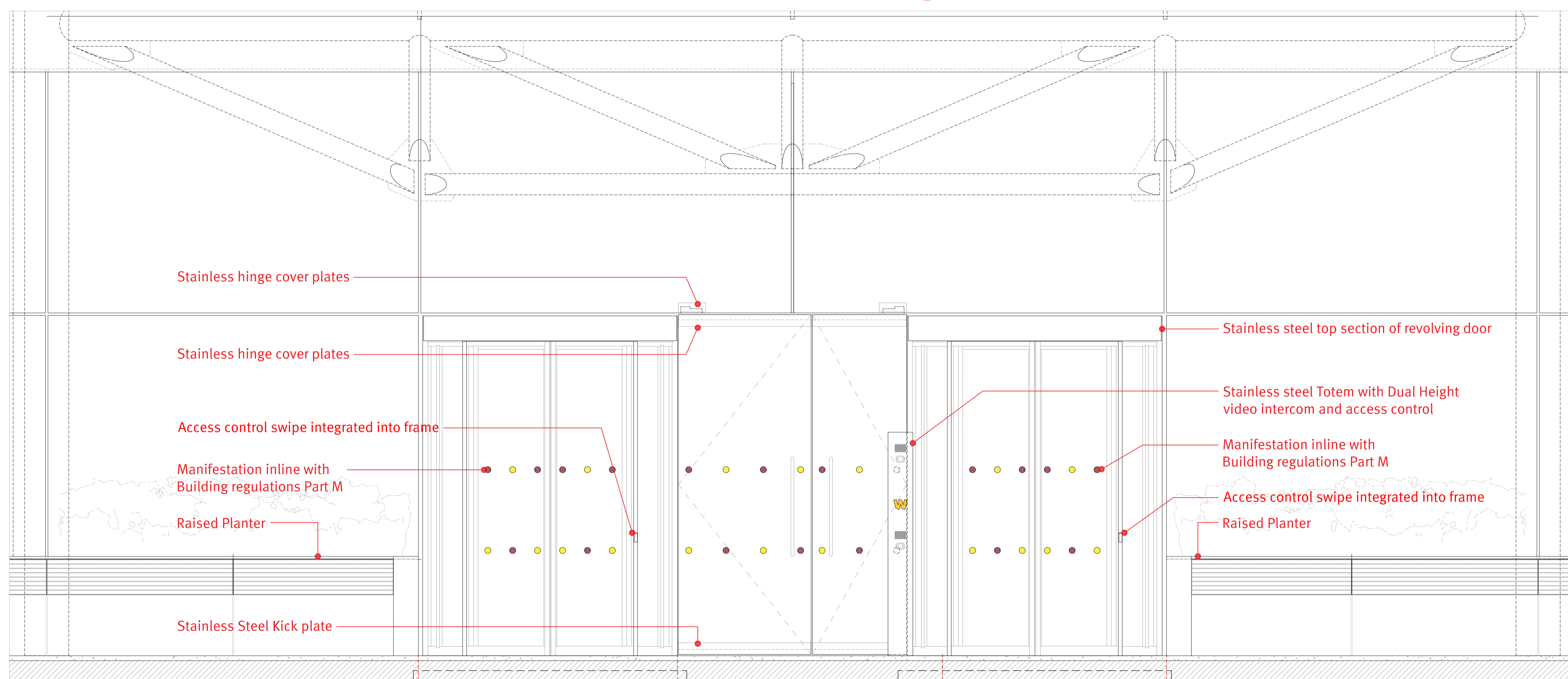
02 Details - Proposed Elevation 1:20 @ A1
