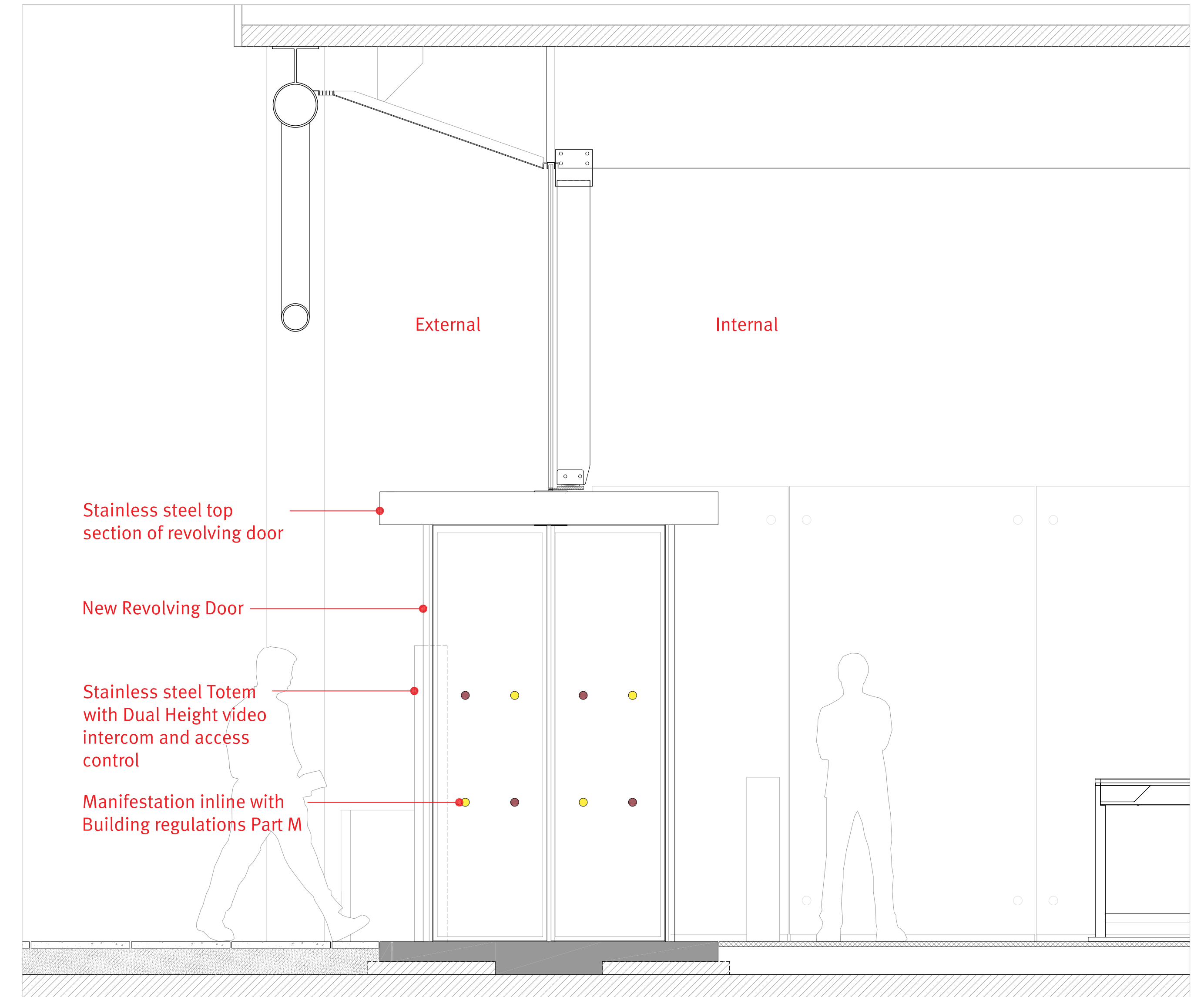
BB Proposed Section - Through Revolving Door 1:20 @ A3
