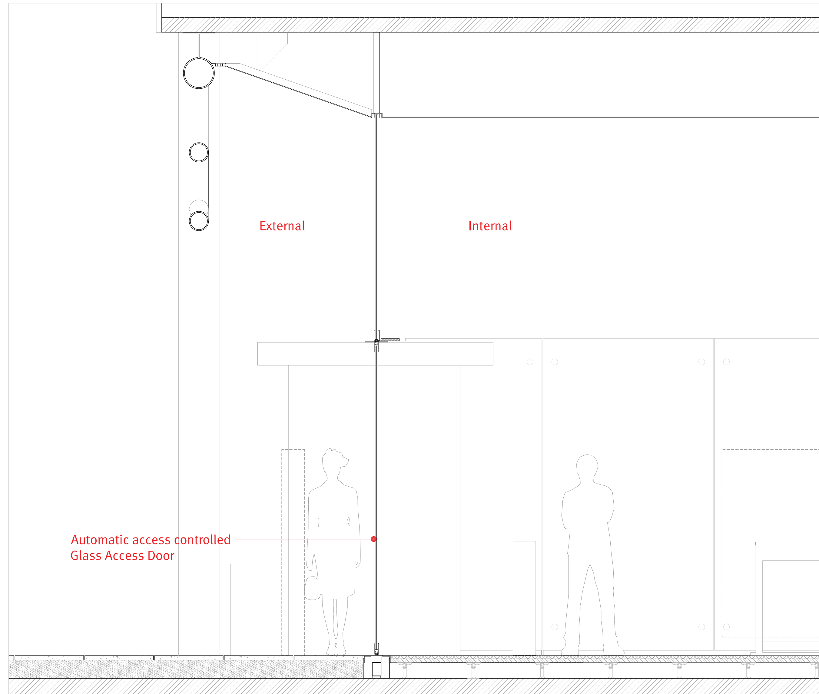
AA Proposed Section - Through Access Door 1:20 @ A3
